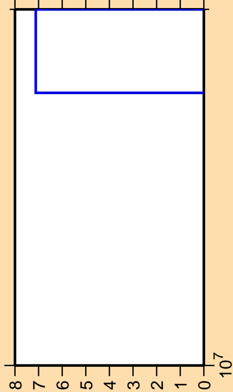
\Delta\sigma/\sigma vs. E for ^{63}\text{Ga}(n,nt)
