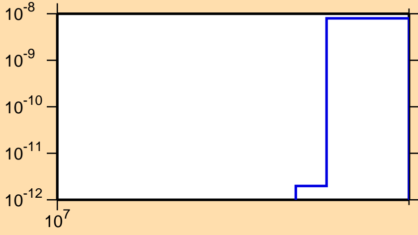
\sigma vs. E for ^{63}\text{Ga} (mt 34)
