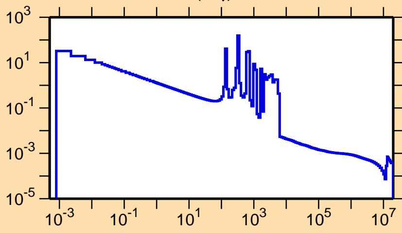
\sigma vs. E for ^{63}\text{Ga}(n,\gamma)
