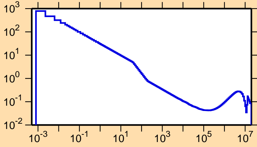
\sigma vs. E for ^{63}\text{Ga}(n,\alpha)
