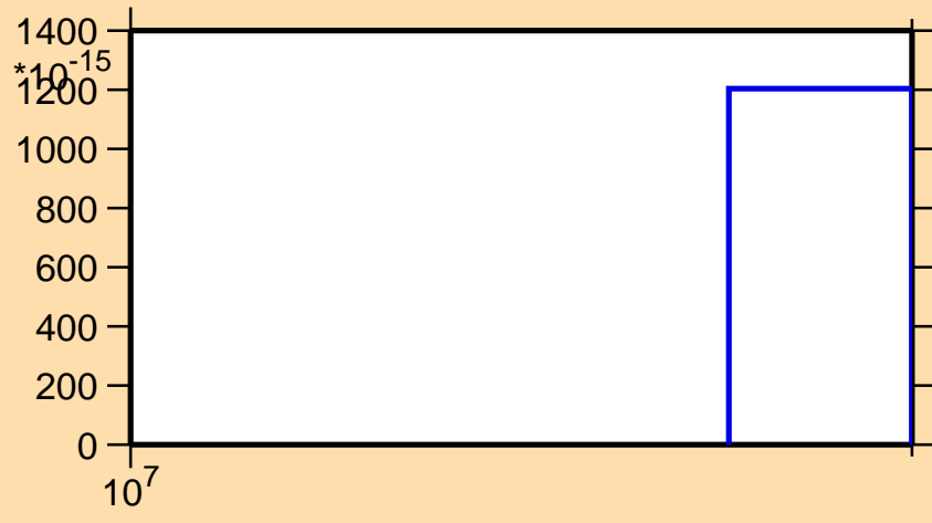
\sigma vs. E for ^{63}\text{Ga}(n,nt)
