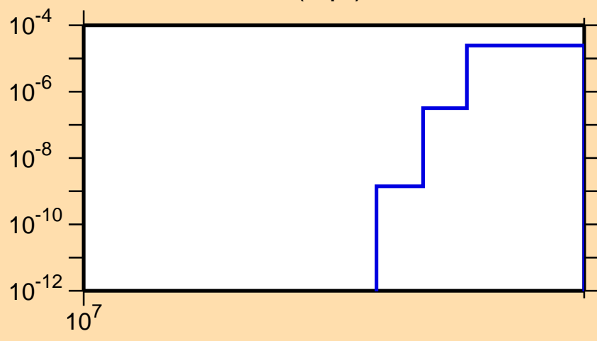
\sigma vs. E for ^{63}\text{Ga}(n,\text{pt})
