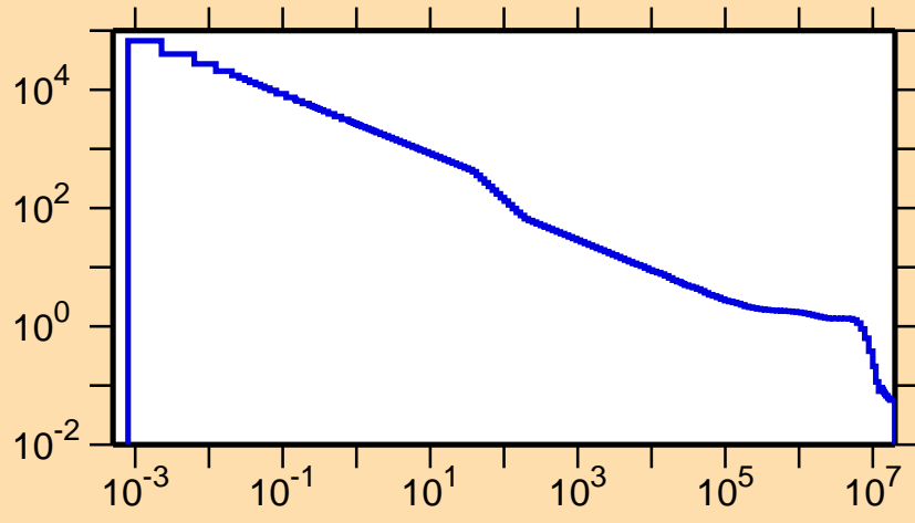
\sigma vs. E for ^{63}\text{Ga}(n,p)
