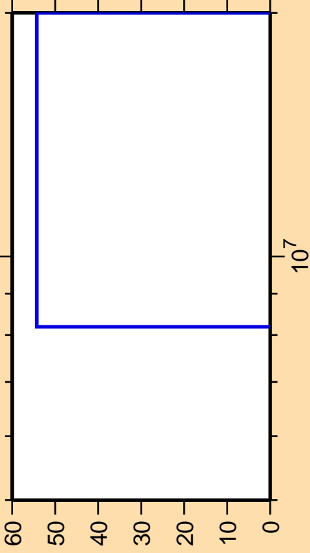
\Delta\sigma/\sigma vs. E for ^{63}\text{Ga}(n,\gamma)
