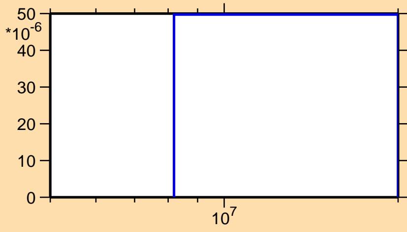
\sigma vs. E for ^{63}\text{Ga}(\text{mt117})
