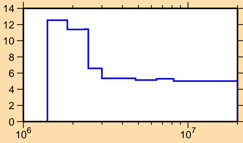
\Delta\sigma/\sigma vs. E for ^{63}\text{Ga}(n,n\text{nonel.})
