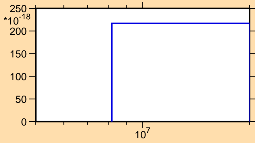
\sigma vs. E for ^{63}\text{Ga}(n,2n\alpha)
