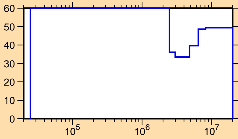
\Delta\sigma/\sigma vs. E for ^{63}\text{Ga}(n,n_1)
