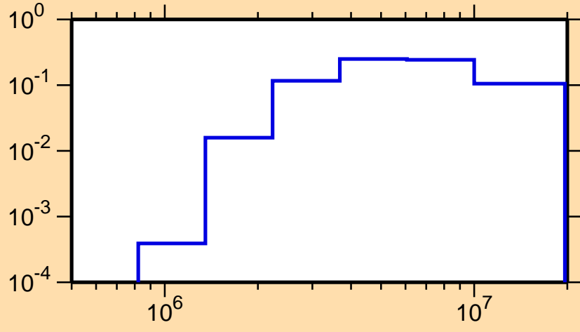
\sigma vs. E for ^{64}\text{Ga}(n,n\text{cont.})
