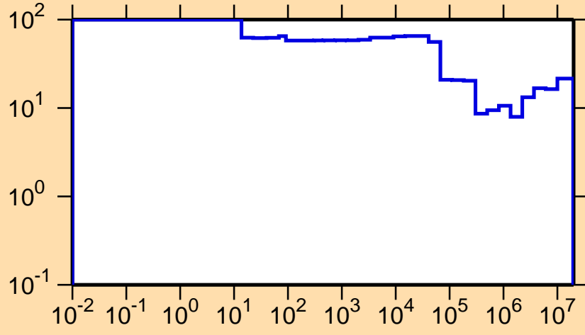
\Delta\sigma/\sigma vs. E for ^{64}\text{Ga}(n,p)
