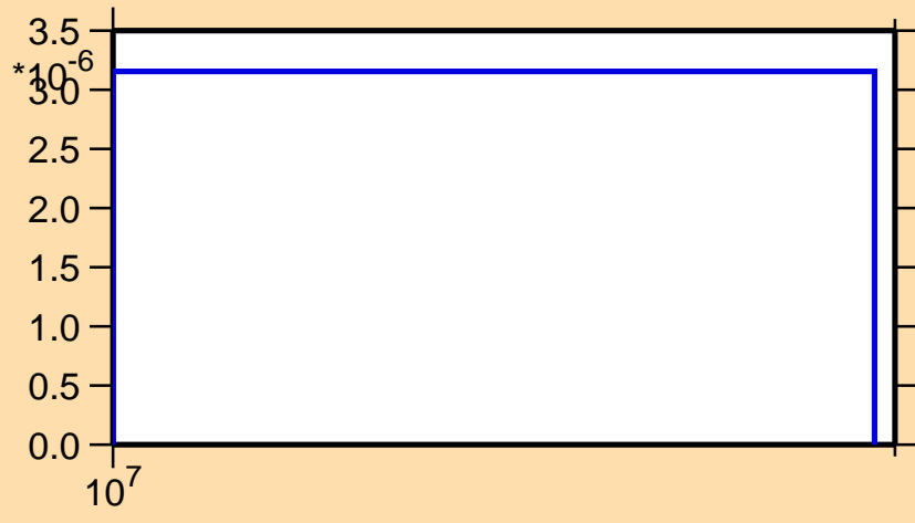
\sigma vs. E for ^{64}\text{Ga}(n,\text{pt})
