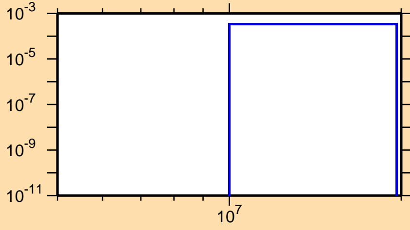
\sigma vs. E for ^{64}\text{Ga}(n,\text{pd})
