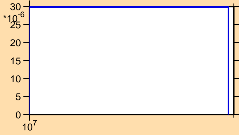
\sigma vs. E for ^{64}\text{Ga}(n,2np)
