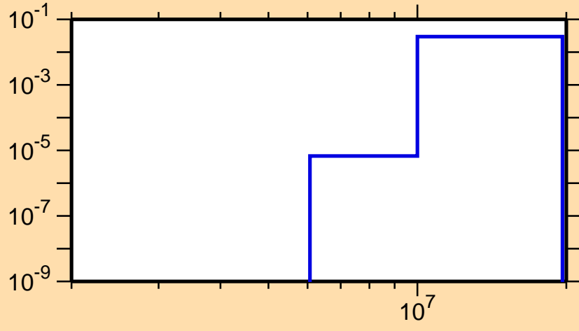
\sigma vs. E for ^{64}\text{Ga}(n,n\alpha)
