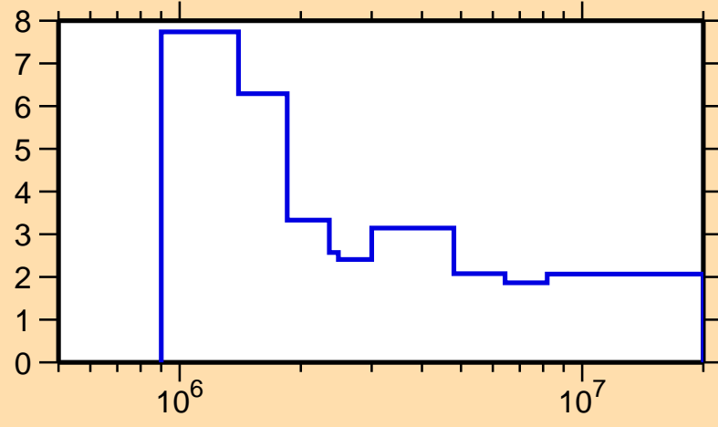
\Delta\sigma/\sigma vs. E for ^{64}\text{Ga}(n,n\text{nonel.})
