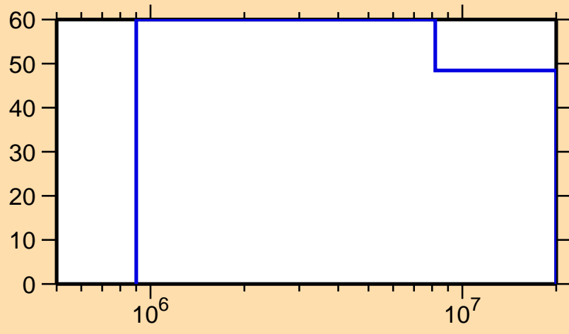
\Delta\sigma/\sigma vs. E for ^{64}\text{Ga}(n,ncont.)
