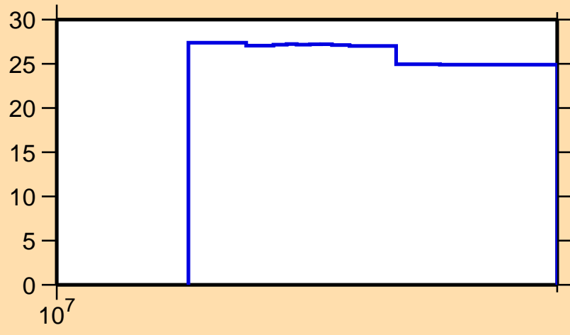
\Delta\sigma/\sigma vs. E for ^{65}\text{Ga}(n,\text{inel.})
