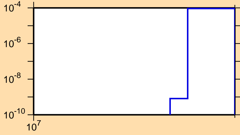
\sigma vs. E for ^{65}\text{Ga}(n,2np)
