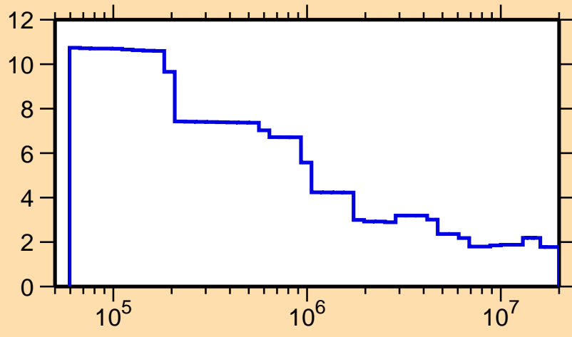
\Delta\sigma/\sigma vs. E for ^{65}\text{Ga}(n,\text{nonel.})
