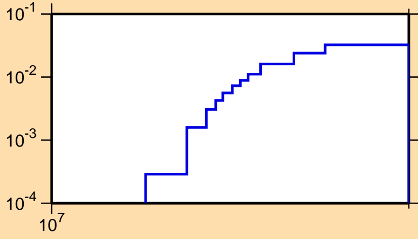
\sigma vs. E for ^{65}\text{Ga}(n,2n)
