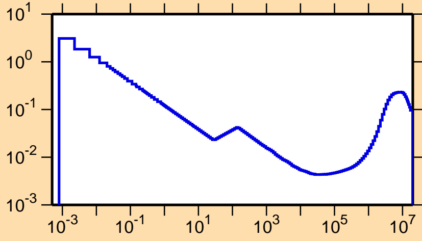
\sigma vs. E for ^{65}\text{Ga}(n,\alpha)
