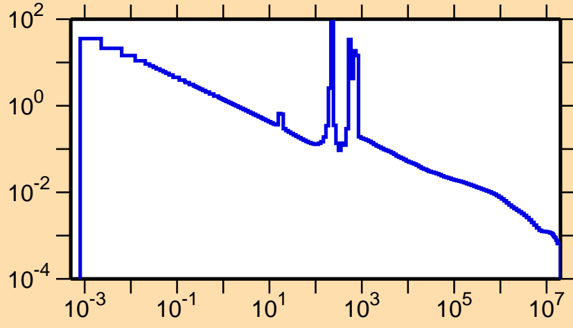
\sigma vs. E for ^{65}\text{Ga}(n,\gamma)
