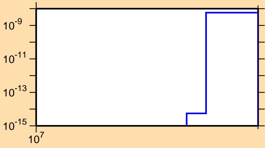
\sigma vs. E for ^{65}\text{Ga}(n,nt)
