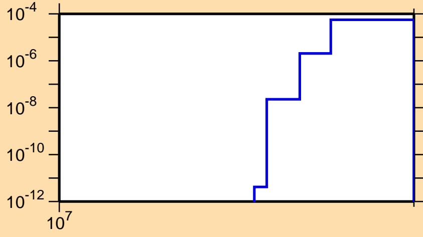
\sigma vs. E for ^{65}\text{Ga}(n,\text{nd})
