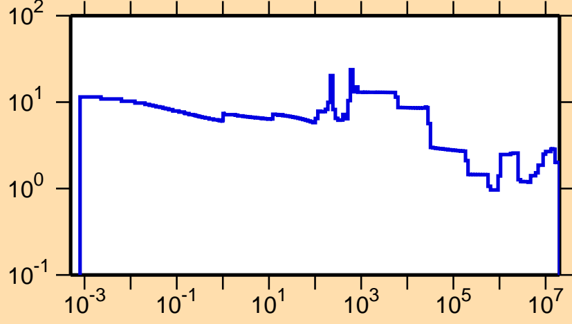
\Delta\sigma/\sigma vs. E for ^{65}\text{Ga}(n,\text{tot.})
