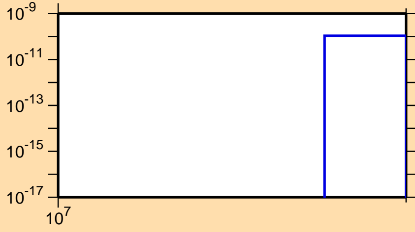
\sigma vs. E for ^{65}\text{Ga}(n,2n\alpha)
