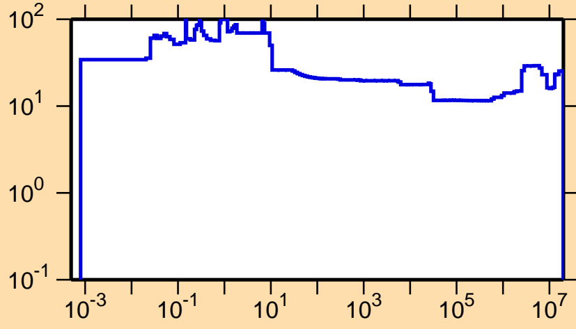
\Delta\sigma/\sigma vs. E for ^{65}\text{Ga}(n,p)
