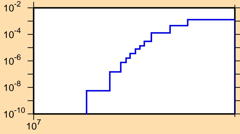
\sigma vs. E for ^{65}\text{Ga}(n,\text{pd})
