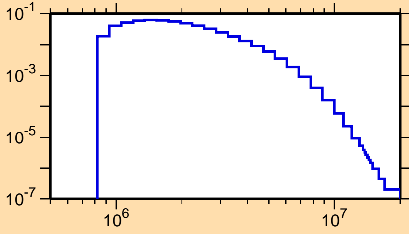
\sigma vs. E for ^{65}\text{Ga}(n,n_4)
