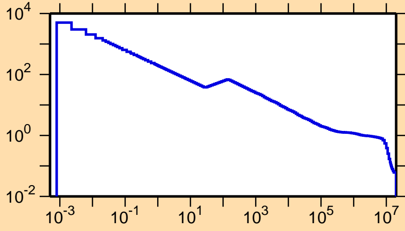
\sigma vs. E for ^{65}\text{Ga}(n,p)
