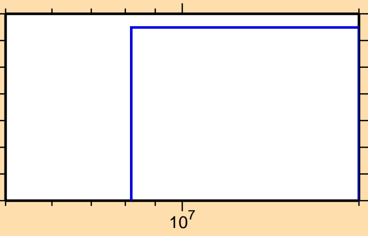
\sigma vs. E for ^{65}\text{Ga}(n,\text{pt})
