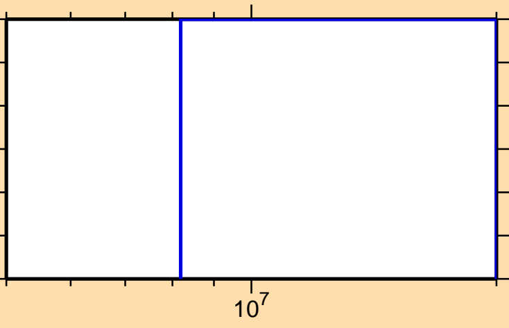
\sigma vs. E for ^{65}\text{Ga}(\text{mt117})
