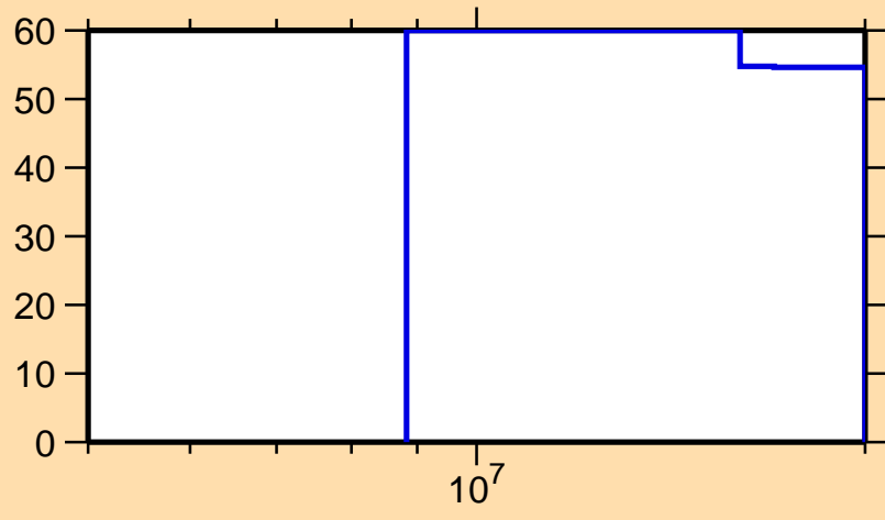
\Delta\sigma/\sigma vs. E for ^{66}\text{Ga}(n,2n)
