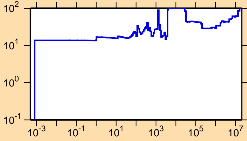
\Delta\sigma/\sigma vs. E for ^{66}\text{Ga}(n,\gamma)
