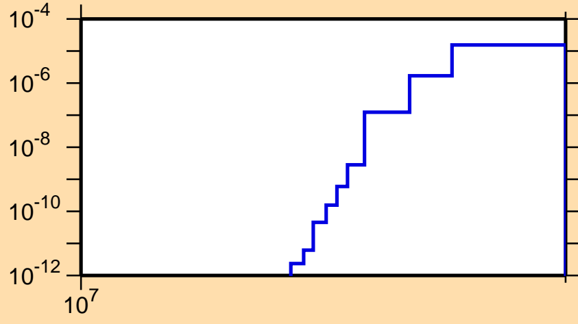
\sigma vs. E for ^{66}\text{Ga}(n,\text{pd})
