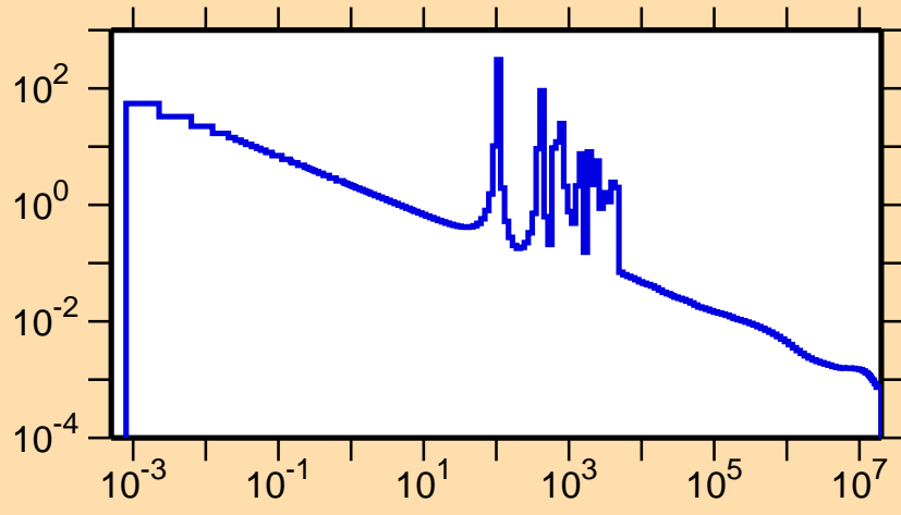
\sigma vs. E for ^{66}\text{Ga}(n,\gamma)
