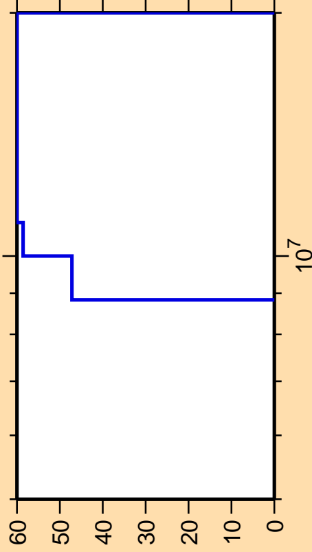
\Delta\sigma/\sigma vs. E for ^{66}\text{Ga}(n,n_1)
