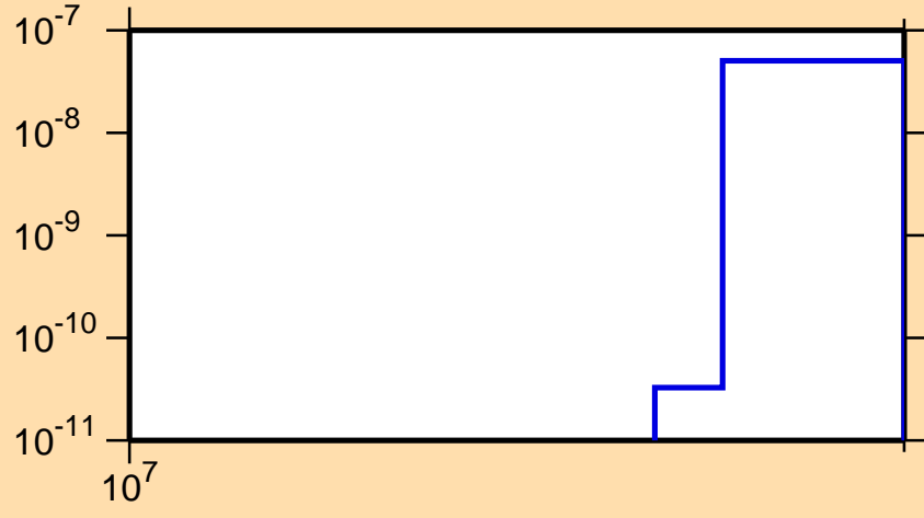
\sigma vs. E for ^{66}\text{Ga} (mt 34)
