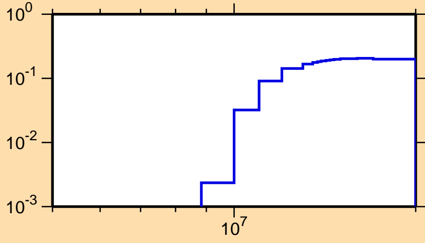
\sigma vs. E for ^{66}\text{Ga}(n,2n)
