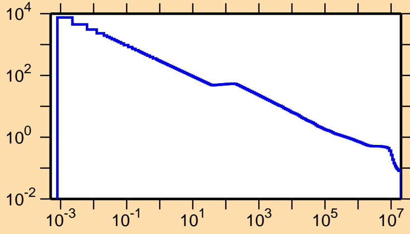
\sigma vs. E for ^{66}\text{Ga}(n,p)
