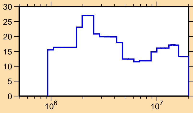
\Delta\sigma/\sigma vs. E for ^{66}\text{Ga}(n,\text{el.})
