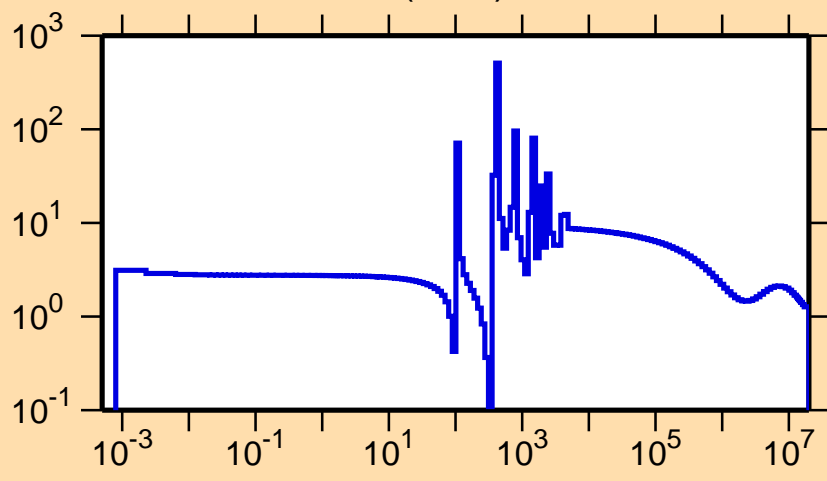
\sigma vs. E for ^{66}\text{Ga}(n,\text{el.})
