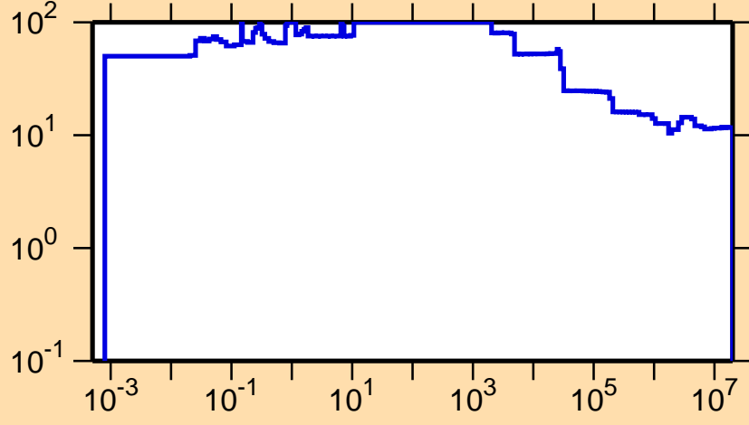
\Delta\sigma/\sigma vs. E for ^{66}\text{Ga}(n,\text{nonel.})
