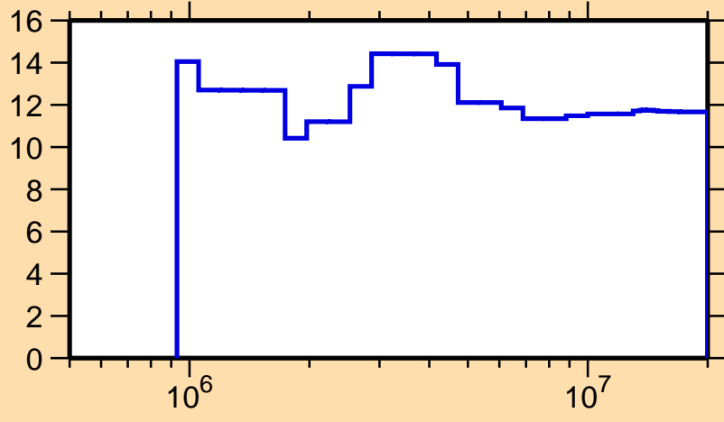
\Delta\sigma/\sigma vs. E for ^{66}\text{Ga}(n,\text{nonel.})
