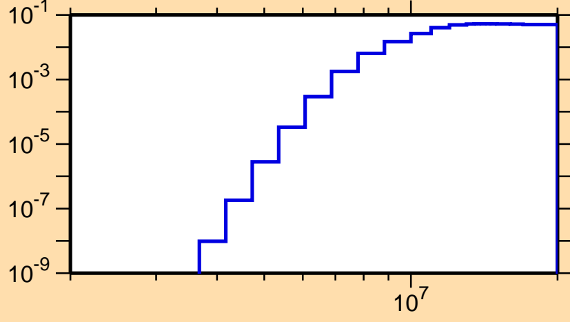
\sigma vs. E for ^{66}\text{Ga}(n,p\alpha)
