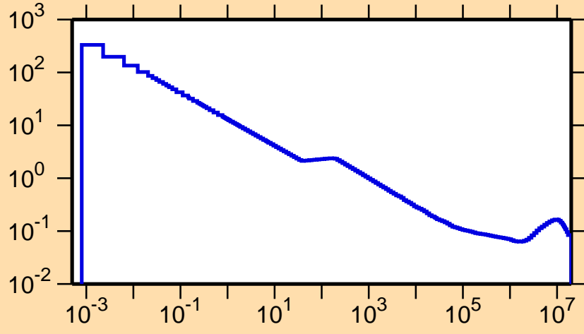
\sigma vs. E for ^{66}\text{Ga}(n,\alpha)
