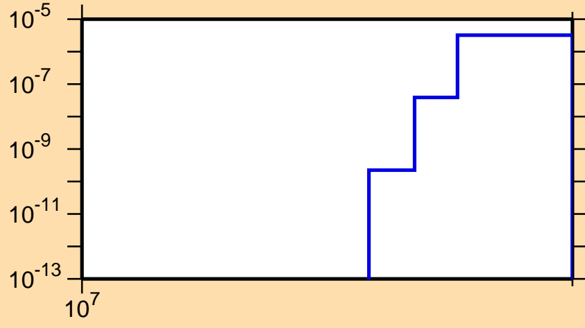
\sigma vs. E for ^{66}\text{Ga}(n,2n\alpha)
