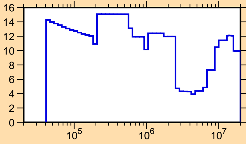
\Delta\sigma/\sigma vs. E for ^{66}\text{Ga}(n,\text{tot.})
