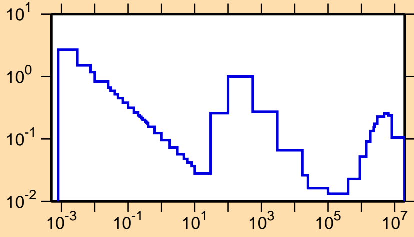
\sigma vs. E for ^{67}\text{Ga}(n,p)
