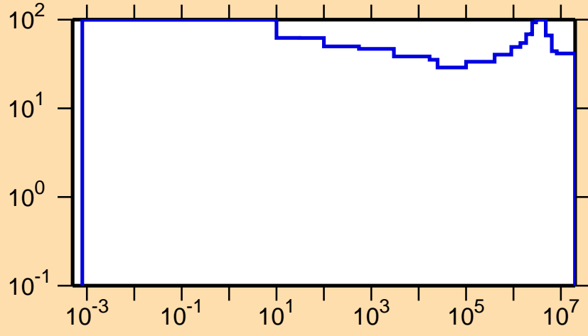
\Delta\sigma/\sigma vs. E for ^{68}\text{Ga}(n,p)
