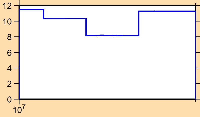
\Delta\sigma/\sigma vs. E for ^{69}\text{Ga}(n,2n)
