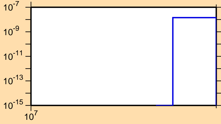
\sigma vs. E for ^{69}\text{Ga}(n,2n\alpha)
