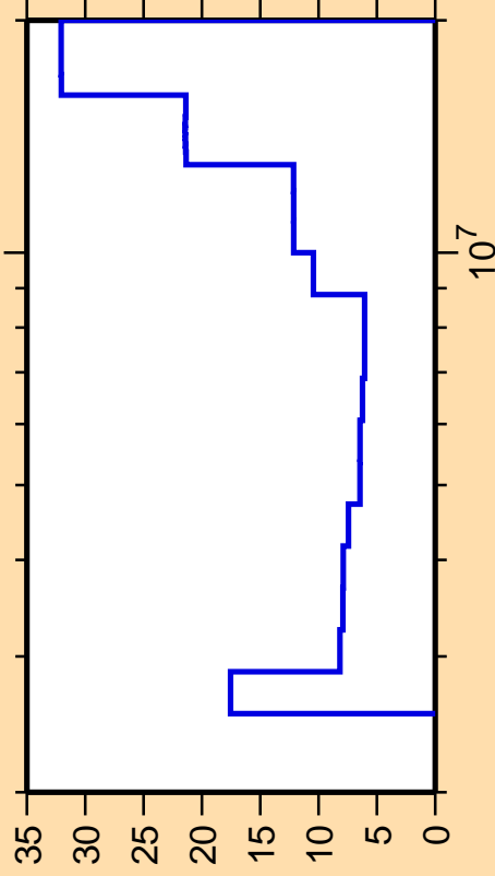
\Delta\sigma/\sigma vs. E for ^{69}\text{Ga}(n,n\text{cont.})
