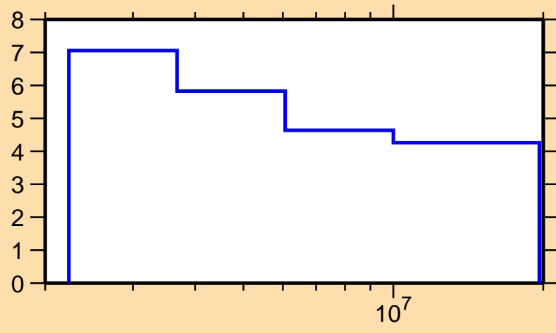
\Delta\sigma/\sigma vs. E for ^{69}\text{Ga}(n,n\text{inel.})
