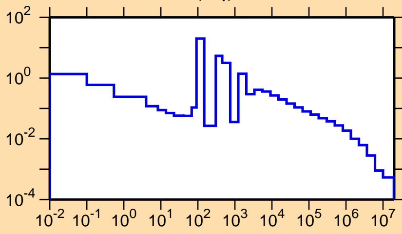
\sigma vs. E for ^{69}\text{Ga}(n,\gamma)
