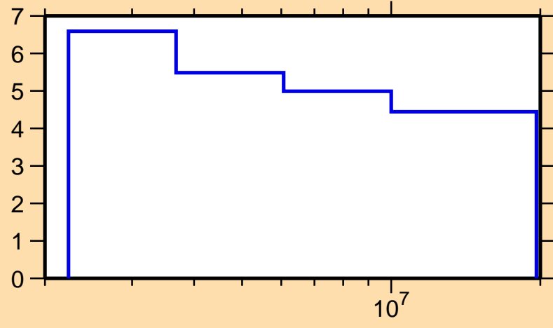
\Delta\sigma/\sigma vs. E for ^{71}\text{Ga}(n,n\text{inel.})
