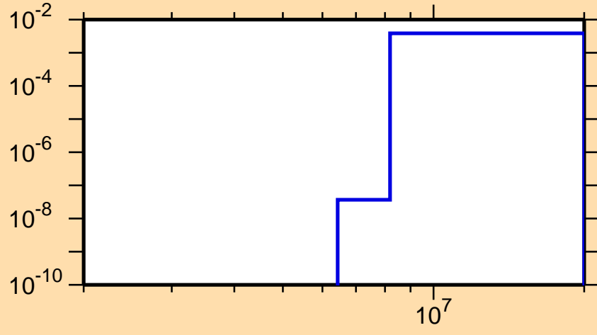
\sigma vs. E for ^{71}\text{Ga}(n,d)
