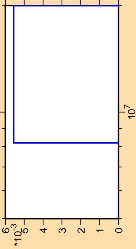
\Delta\sigma/\sigma vs. E for ^{71}\text{Ga}(\text{mt117})
