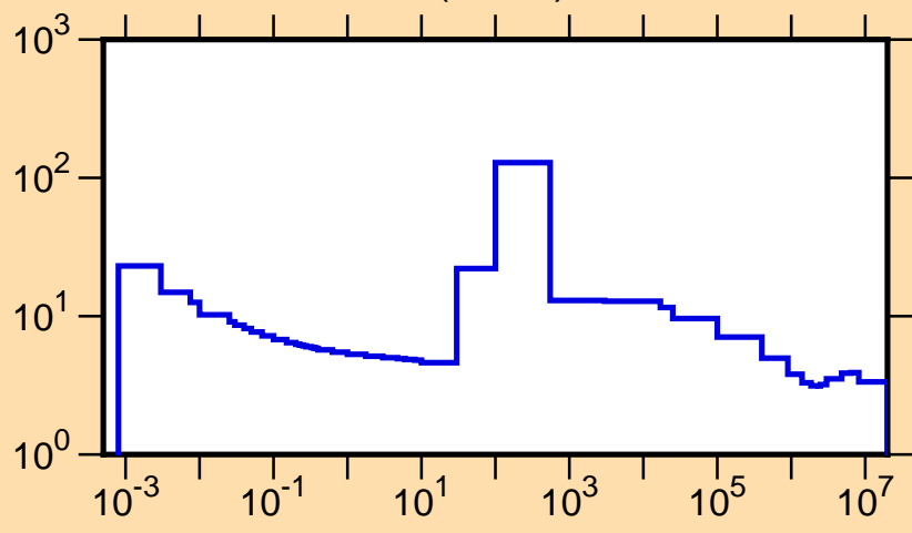
\sigma vs. E for ^{71}\text{Ga}(n,\text{tot.})
