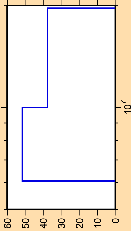
\Delta\sigma/\sigma vs. E for ^{72}\text{Ga}(n,np)
