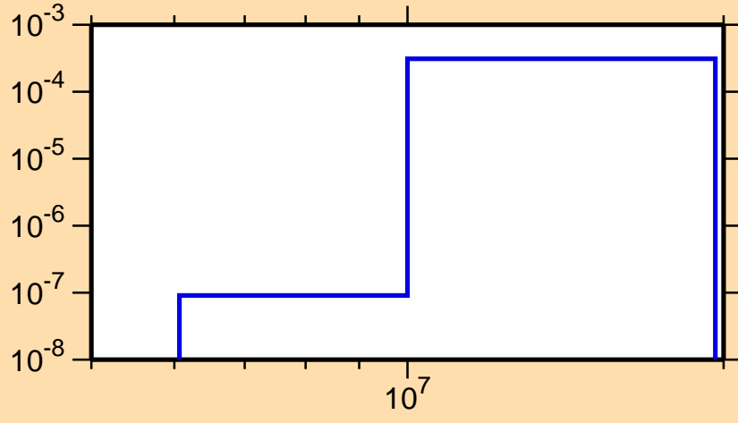
\sigma vs. E for ^{72}\text{Ga}(n,t)
