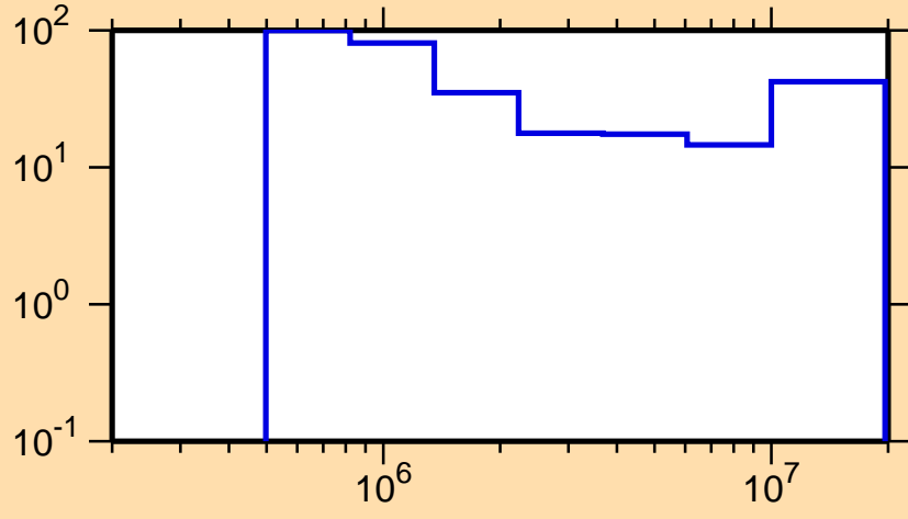
\Delta\sigma/\sigma vs. E for ^{72}\text{Ga}(n,n\text{cont.})
