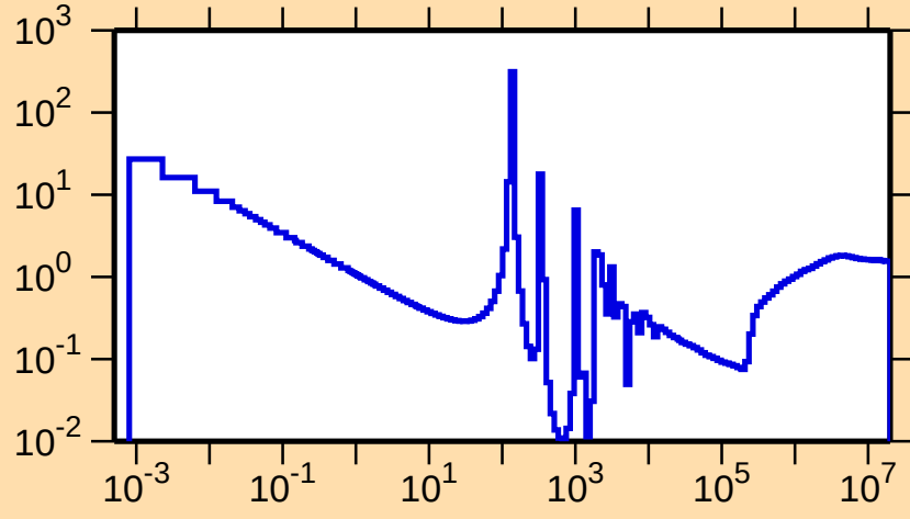
\sigma vs. E for ^{73}\text{Ga}(n,\text{nonel.})
