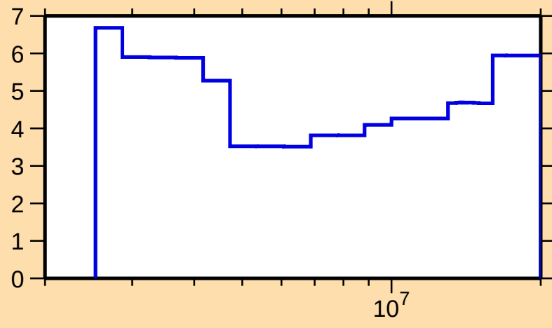
\Delta\sigma/\sigma vs. E for ^{73}\text{Ga}(\text{n},\text{nonel.})
