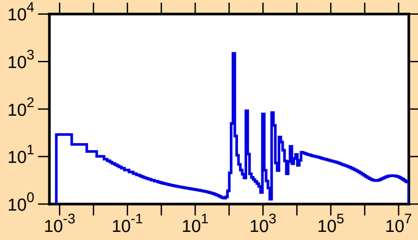
\sigma vs. E for ^{73}\text{Ga}(n,\text{tot.})
