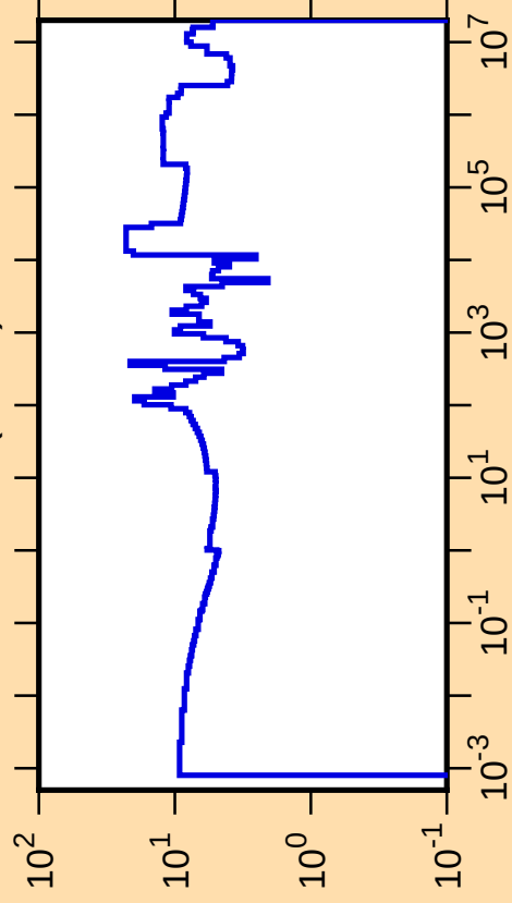
\Delta\sigma/\sigma vs. E for ^{73}\text{Ga}(n,\text{tot.})
