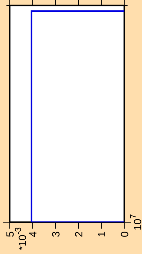
\Delta\sigma/\sigma vs. E for ^{73}\text{Ga}(n,\text{He}3)
