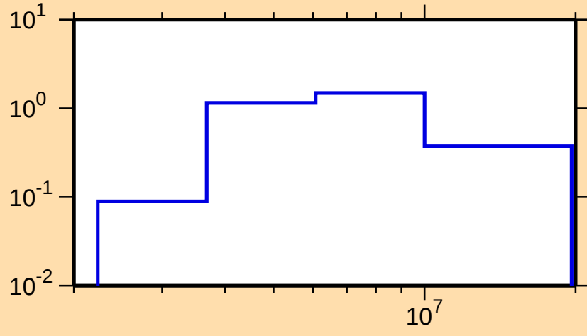
\sigma vs. E for ^{73}\text{Ga}(n,n\text{cont.})
