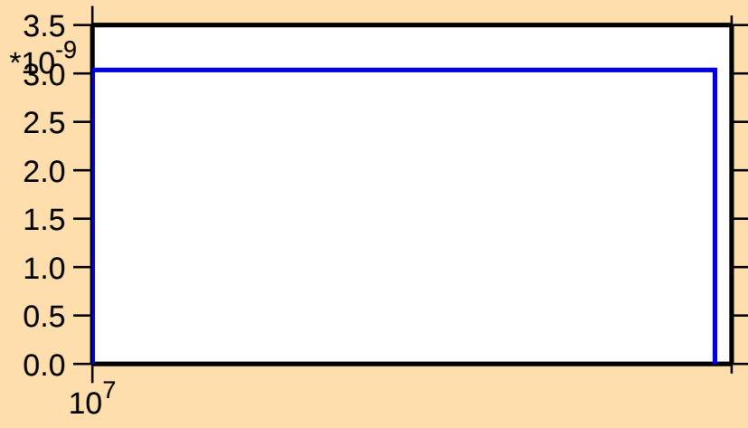
\sigma vs. E for ^{73}\text{Ga}(n,\text{nt})
