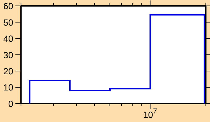
\Delta\sigma/\sigma vs. E for ^{73}\text{Ga}(n,n\text{cont.})
