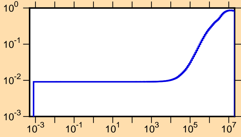
\mu vs. E for ^{74}\text{Ga}(\text{mt251})
