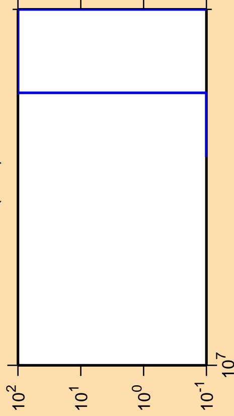
\Delta\sigma/\sigma vs. E for ^{74}\text{Ga}(n,\text{nt})
