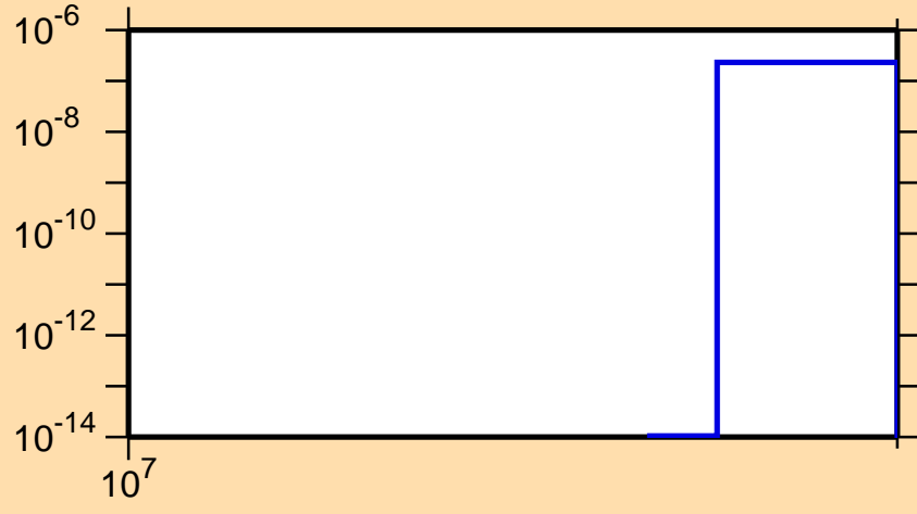
\sigma vs. E for ^{74}\text{Ga}(n,\text{nt})
