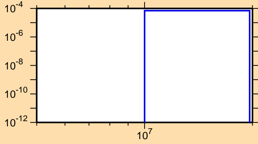
\sigma vs. E for ^{74}\text{Ga}(n,n\alpha)
