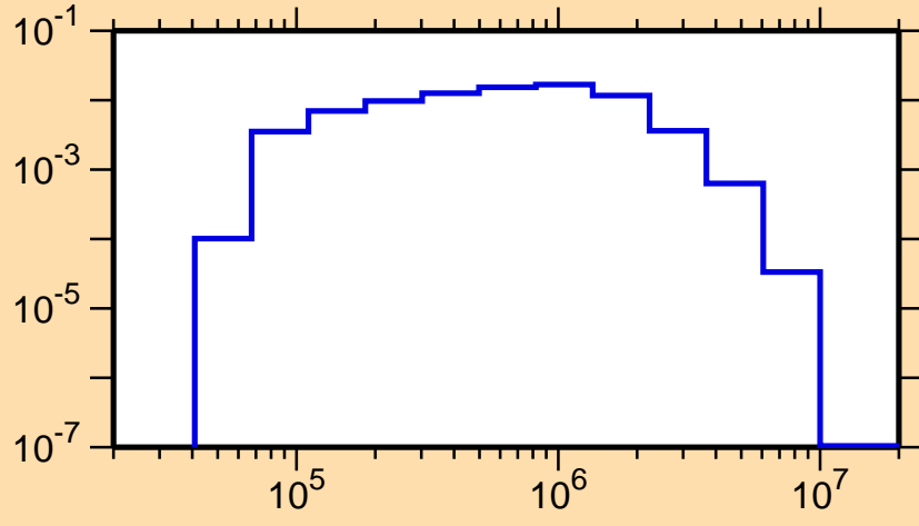
\sigma vs. E for ^{74}\text{Ga}(n,n_2)
