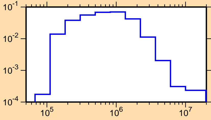
\sigma vs. E for ^{74}\text{Ga}(n,n_3)
