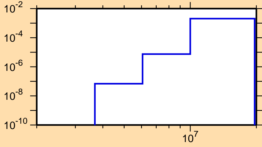
\sigma vs. E for ^{74}\text{Ga}(n,\alpha)
