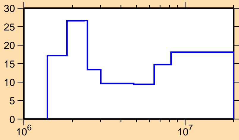
\Delta\sigma/\sigma vs. E for ^{74}\text{Ga}(n,el.)
