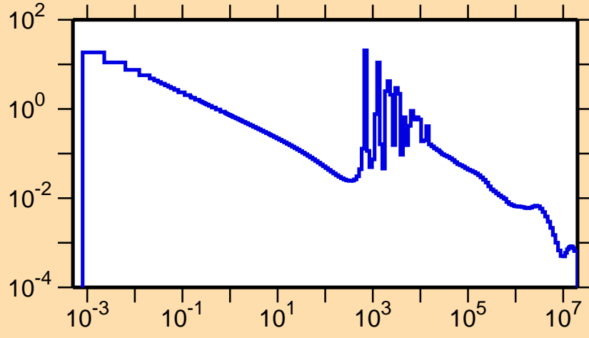
\sigma vs. E for ^{75}\text{Ga}(n,\gamma)
