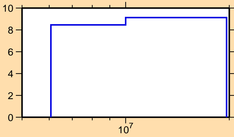
\Delta\sigma/\sigma vs. E for ^{75}\text{Ga}(n,\text{nonel.})
