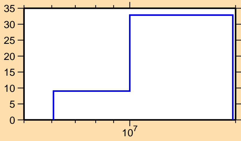
\Delta\sigma/\sigma vs. E for ^{75}\text{Ga}(n,n\text{cont.})
