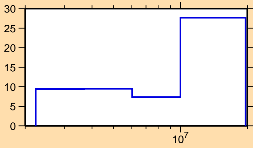
\Delta\sigma/\sigma vs. E for ^{75}\text{Ga}(n,\text{inel.})
