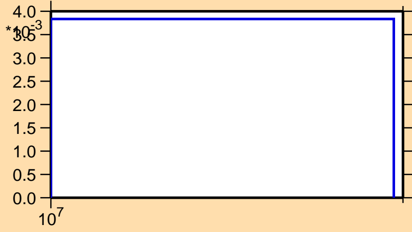
\sigma vs. E for ^{75}\text{Ga}(n,3n)
