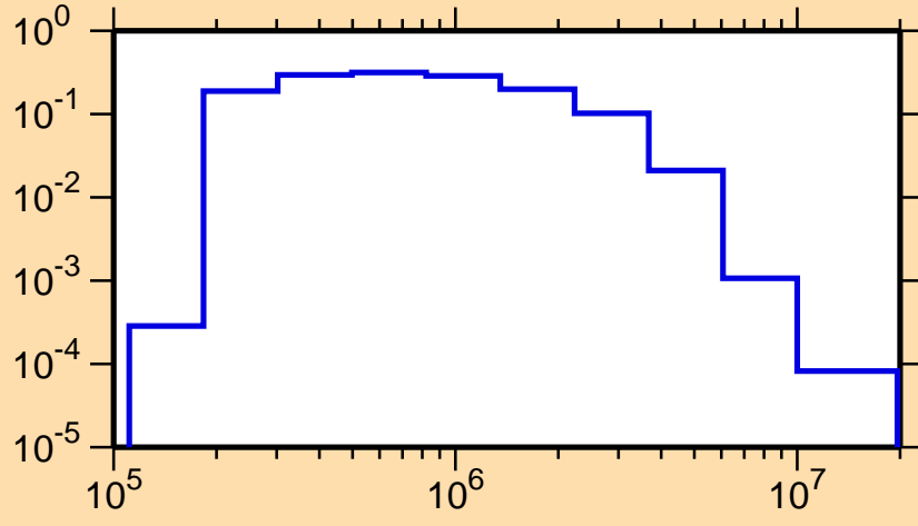
\sigma vs. E for ^{75}\text{Ga}(n,n_2)
