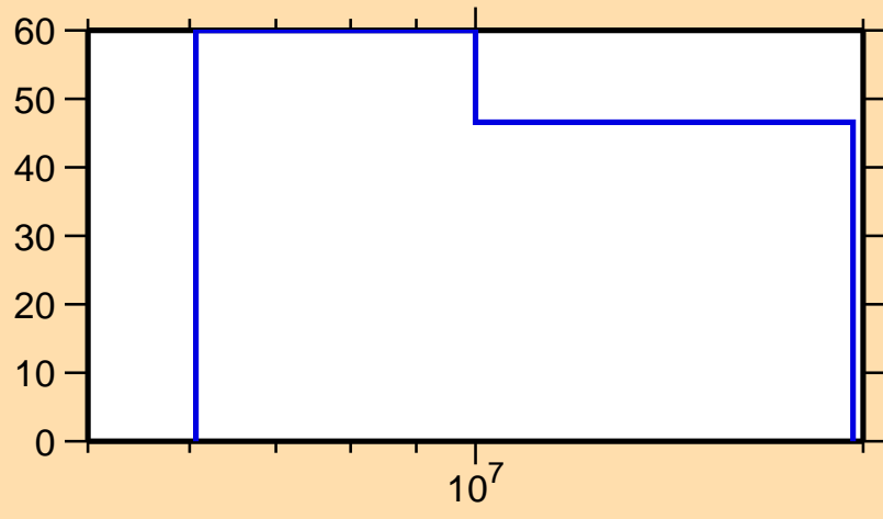
\Delta\sigma/\sigma vs. E for ^{75}\text{Ga}(n,p)
