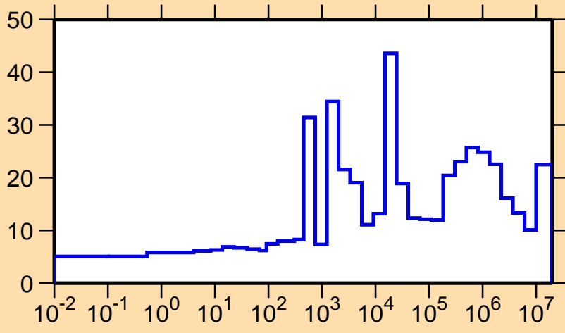
\Delta\sigma/\sigma vs. E for ^{75}\text{Ga}(n,\text{el.})
