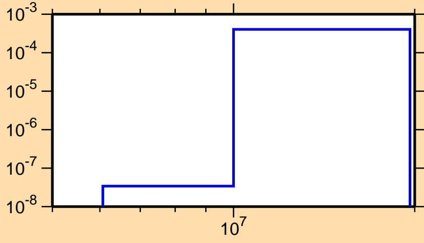
\sigma vs. E for ^{75}\text{Ga}(n,\alpha)
