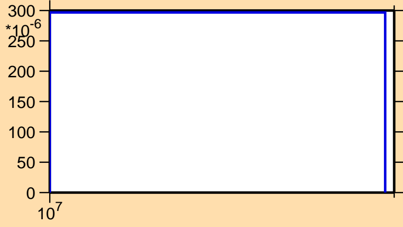
\sigma vs. E for ^{75}\text{Ga}(n,np)
