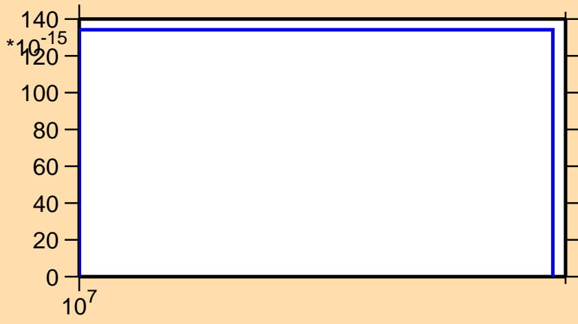
\sigma vs. E for ^{75}\text{Ga}(n,2np)
