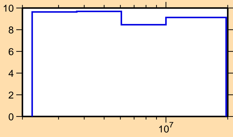
\Delta\sigma/\sigma vs. E for ^{75}\text{Ga}(n,n\text{inel.})
