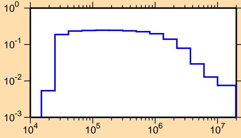
\sigma vs. E for ^{75}\text{Ga}(n,n_1)
