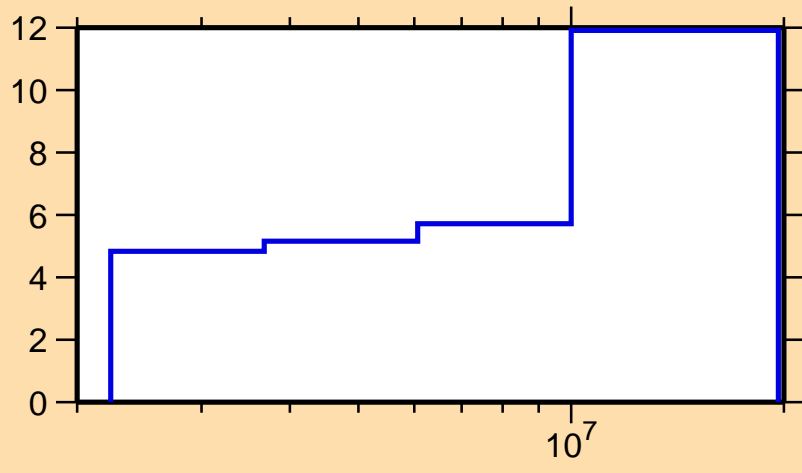
\Delta\sigma/\sigma vs. E for ^{75}\text{Ga}(n,\text{tot.})
