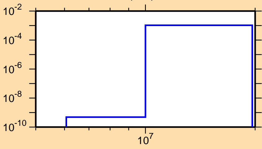
\sigma vs. E for ^{75}\text{Ga}(n,d)
