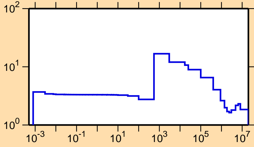
\sigma vs. E for ^{75}\text{Ga}(n,\text{el.})
