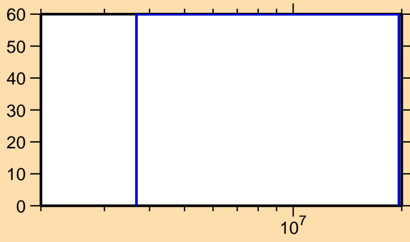
\Delta\sigma/\sigma vs. E for ^{76}\text{Ga}(n,n_1)
