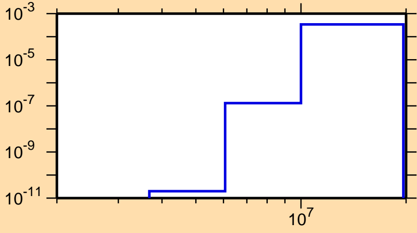
\sigma vs. E for ^{76}\text{Ga}(n,\alpha)
