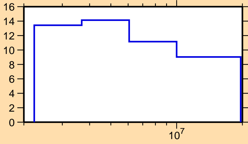
\Delta\sigma/\sigma vs. E for ^{76}\text{Ga}(n,n\text{onel.})
