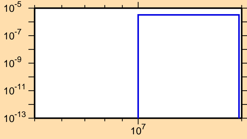
\sigma vs. E for ^{76}\text{Ga}(n,n\alpha)
