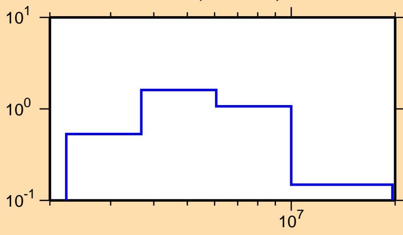
\sigma vs. E for ^{76}\text{Ga}(n,n\text{cont.})
