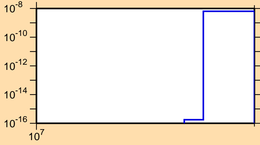
\sigma vs. E for ^{78}\text{Ga}(n,2np)
