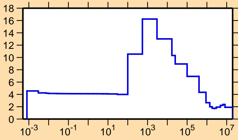
\sigma vs. E for ^{78}\text{Ga}(n,\text{el.})
