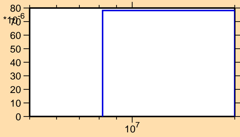
\sigma vs. E for ^{78}\text{Ga}(n,d)
