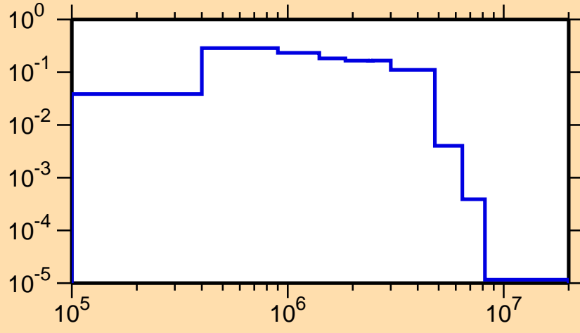
\sigma vs. E for ^{78}\text{Ga}(n,n_1)
