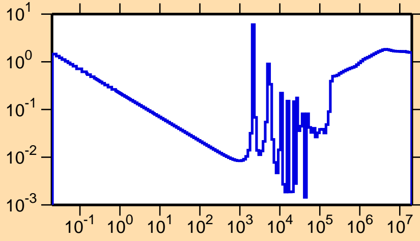
\sigma vs. E for ^{79}\text{Ga}(n,\text{nonel.})
