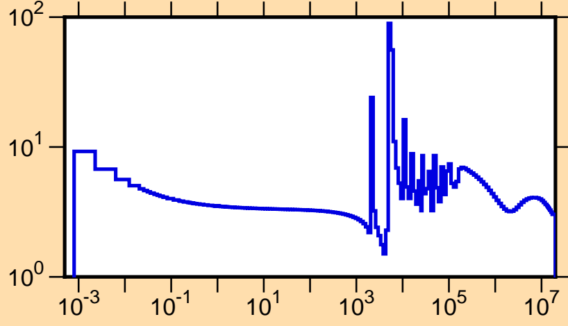
\sigma vs. E for ^{79}\text{Ga}(n,\text{tot.})
