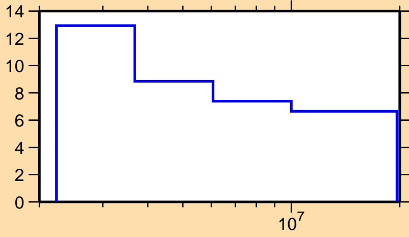
\Delta\sigma/\sigma vs. E for ^{79}\text{Ga}(n,n\text{nonel.})
