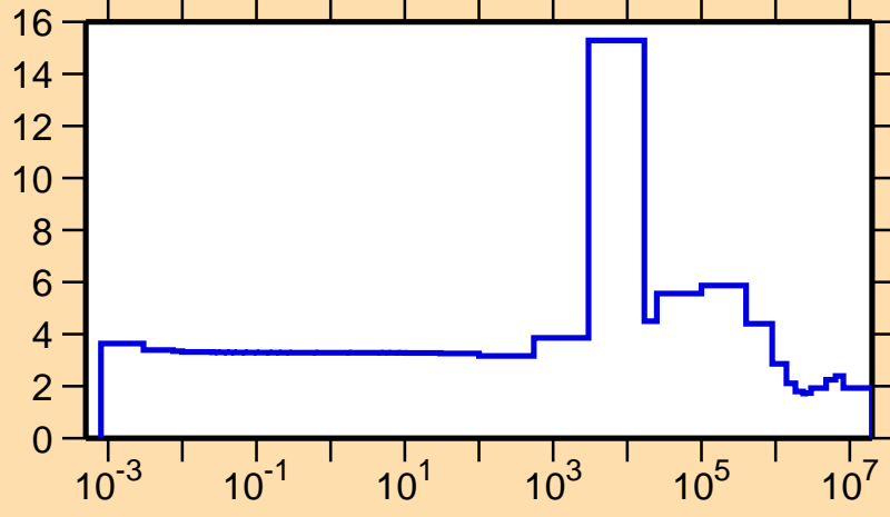
\sigma vs. E for ^{79}\text{Ga}(n,\text{el.})
