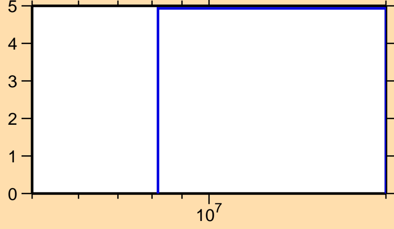
\Delta\sigma/\sigma vs. E for ^{79}\text{Ga}(n,2n)
