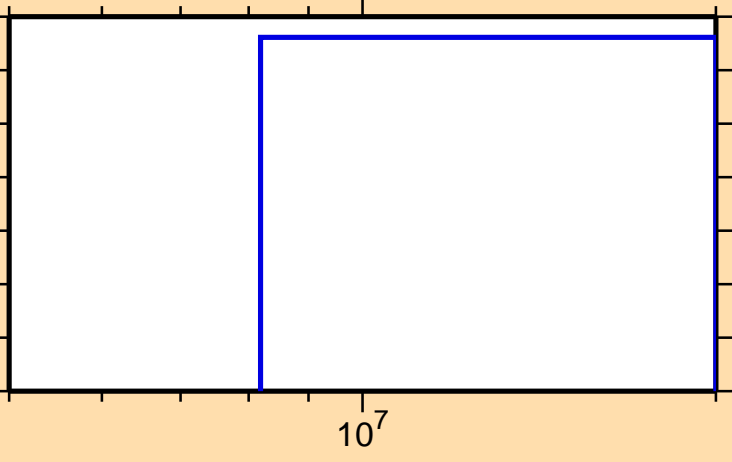
\sigma vs. E for ^{79}\text{Ga}(n,3n)
