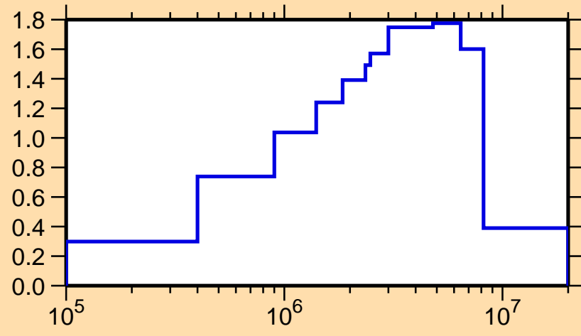
\sigma vs. E for ^{79}\text{Ga}(n,\text{inel.})
