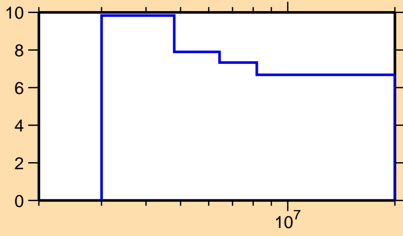
\Delta\sigma/\sigma vs. E for ^{79}\text{Ga}(n,n\text{onel.})
