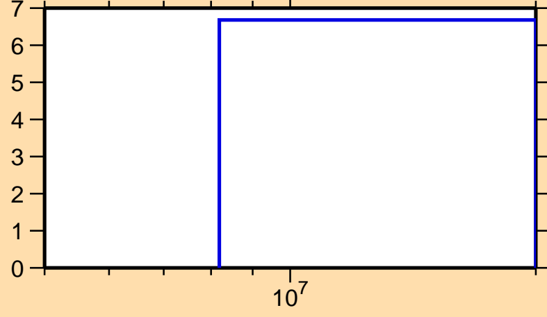
\Delta\sigma/\sigma vs. E for ^{79}\text{Ga}(n,\text{nonel.})
