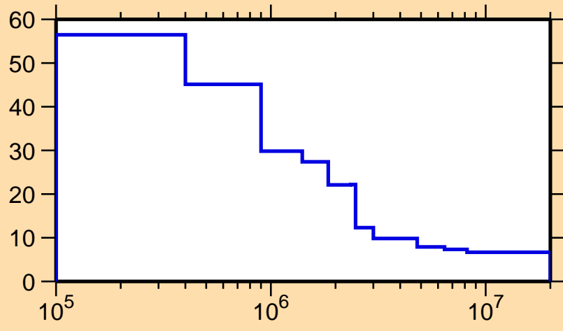
\Delta\sigma/\sigma vs. E for ^{79}\text{Ga}(n,\text{nonel.})
