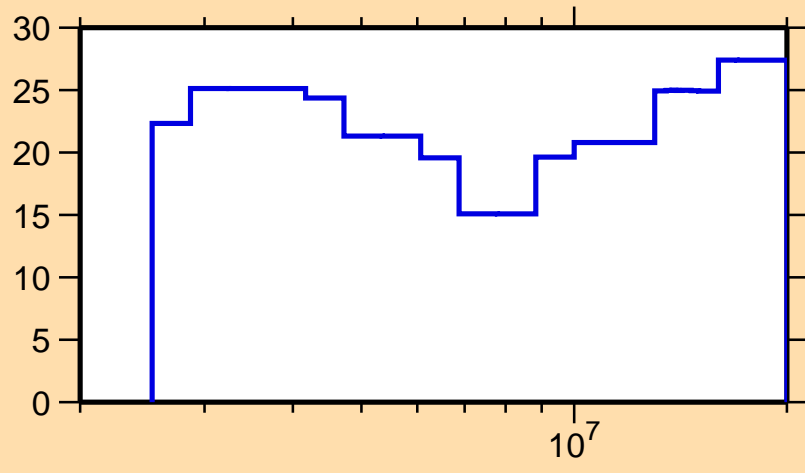
\Delta\sigma/\sigma vs. E for ^{80}\text{Ga}(n,n\text{onel.})
