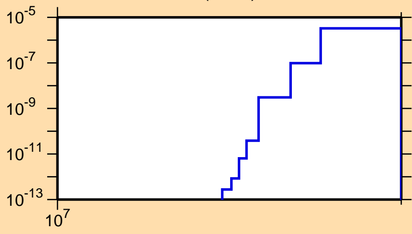
\sigma vs. E for ^{80}\text{Ga}(n,\alpha)
