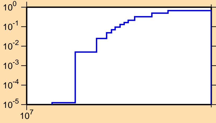
\sigma vs. E for ^{80}\text{Ga}(n,3n)
