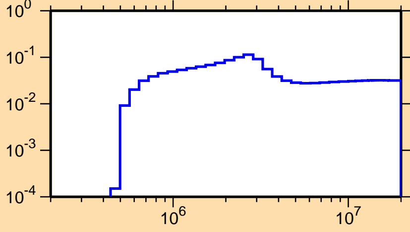
\sigma vs. E for ^{80}\text{Ga}(n,n_3)
