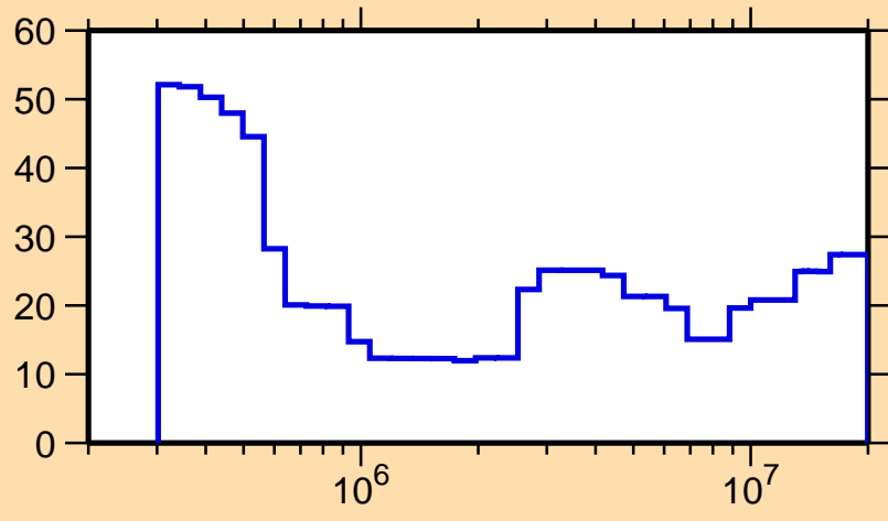
\Delta\sigma/\sigma vs. E for ^{80}\text{Ga}(n,\text{nonel.})
