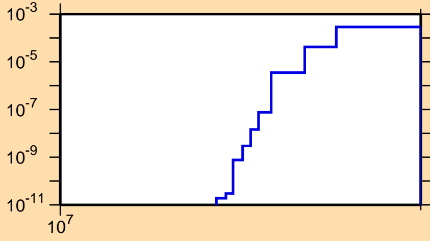
\sigma vs. E for ^{80}\text{Ga}(n,np)
