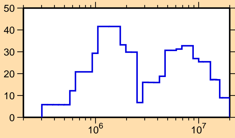
\Delta\sigma/\sigma vs. E for ^{80}\text{Ga}(n,\text{tot.})
