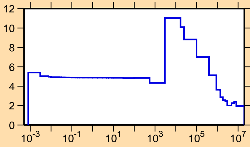
\sigma vs. E for ^{80}\text{Ga}(n,\text{el.})
