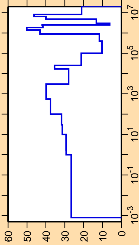
\Delta\sigma/\sigma vs. E for ^{80}\text{Ga}(n,\text{el.})
