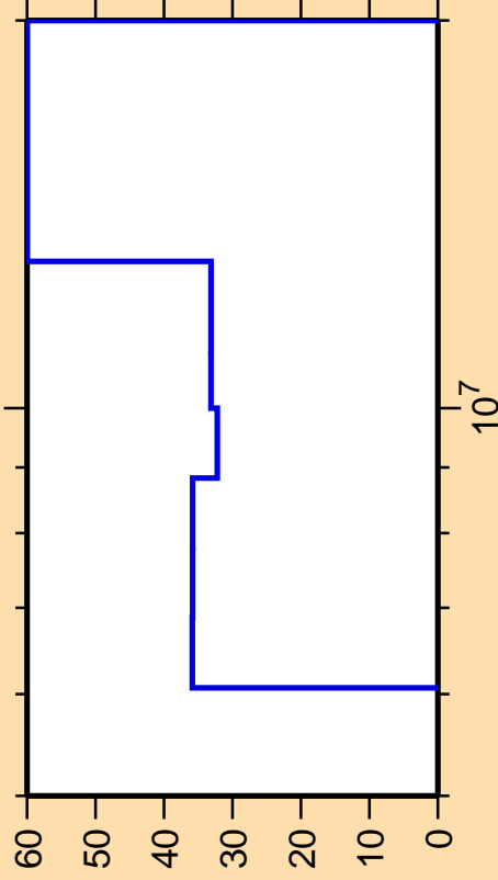
\Delta\sigma/\sigma vs. E for ^{81}\text{Ga}(n,2n)
