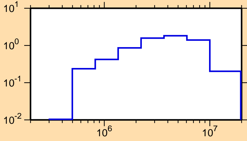
\sigma vs. E for ^{81}\text{Ga}(n,\text{inel.})
