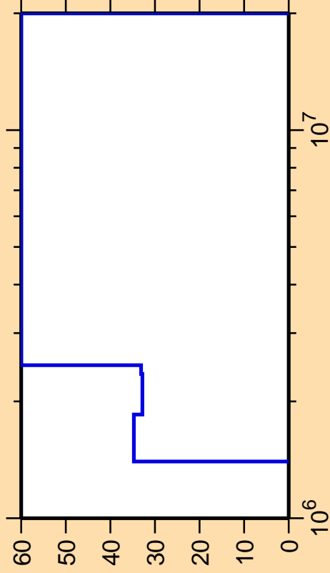
\Delta\sigma/\sigma vs. E for ^{81}\text{Ga}(n,n_4)
