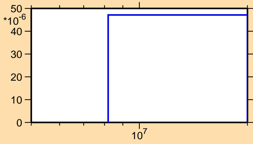
\sigma vs. E for ^{81}\text{Ga}(n,p)
