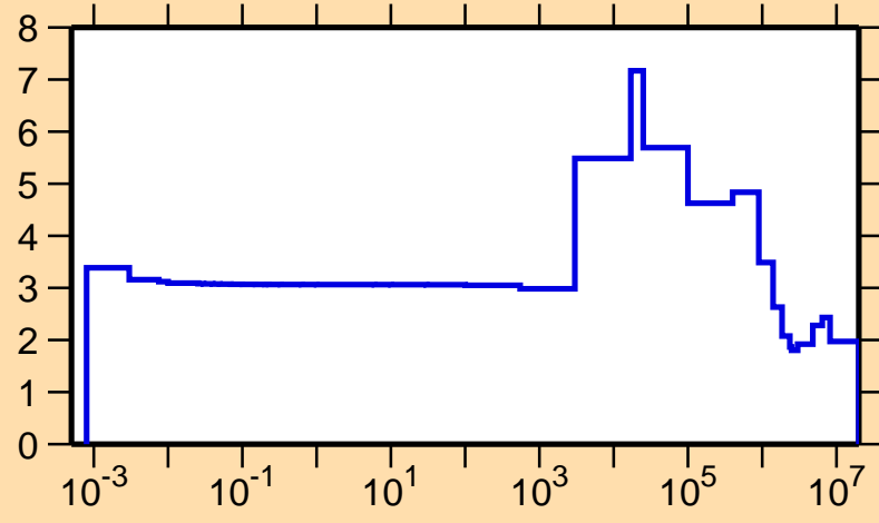
\sigma vs. E for ^{81}\text{Ga}(n,\text{el.})
