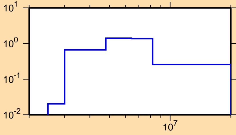
\sigma vs. E for ^{81}\text{Ga}(n,n\text{cont.})
