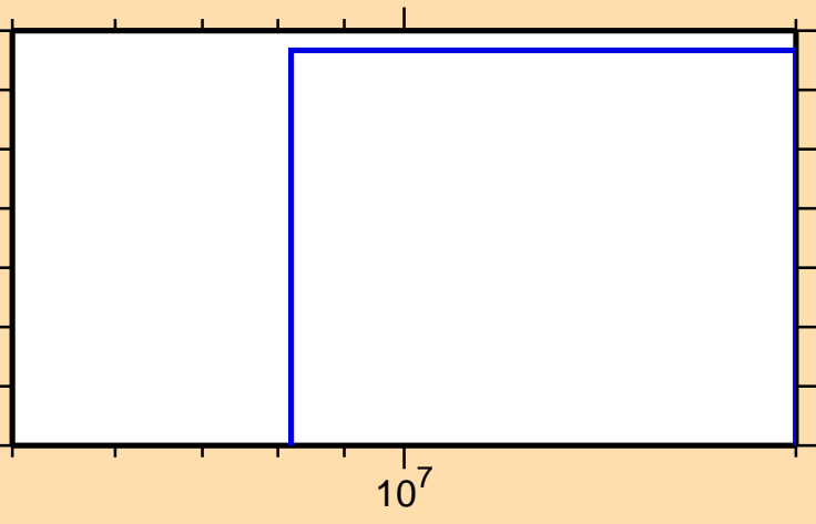
\sigma vs. E for ^{81}\text{Ga}(n,\alpha)
