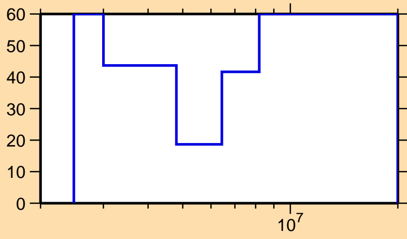
\Delta\sigma/\sigma vs. E for ^{81}\text{Ga}(n,n\text{cont.})
