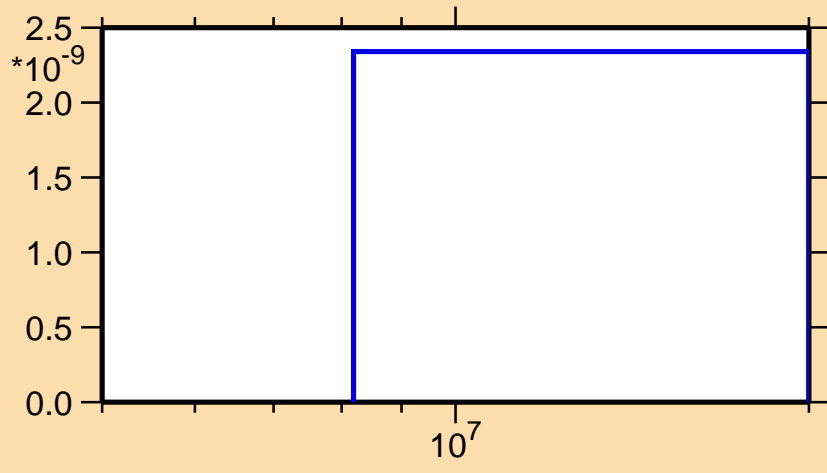
\sigma vs. E for ^{81}\text{Ga}(n,nt)
