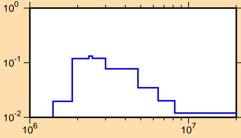
\sigma vs. E for ^{81}\text{Ga}(n,n_4)
