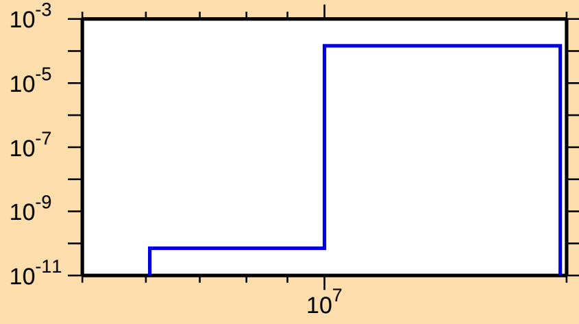
\sigma vs. E for ^{135}\text{Gd}(n,t)
