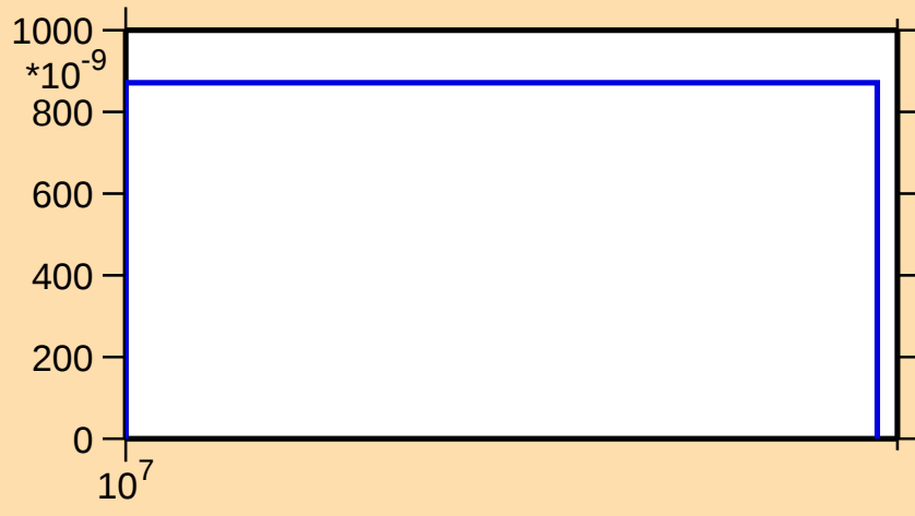
\sigma vs. E for ^{135}\text{Gd}(n,2np)
