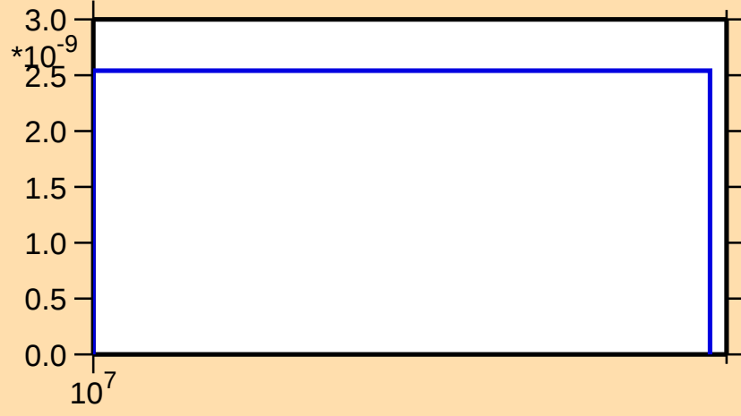
\sigma vs. E for ^{135}\text{Gd}(n,\text{nd})
