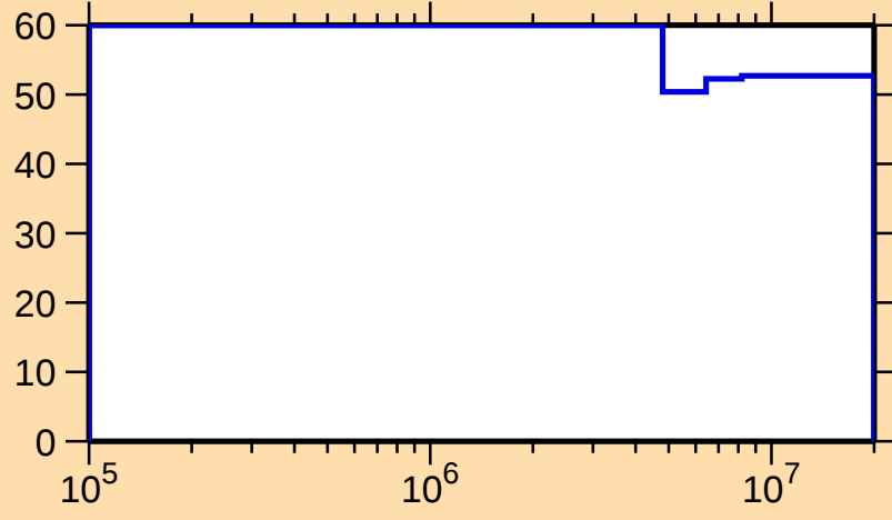
\Delta\sigma/\sigma vs. E for ^{135}\text{Gd}(n,n\text{cont.})
