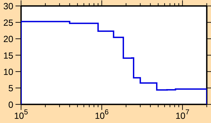
\Delta\sigma/\sigma vs. E for ^{135}\text{Gd}(n,\text{nonel.})
