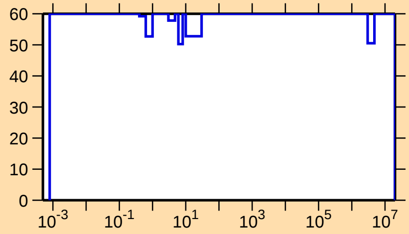
\Delta\sigma/\sigma vs. E for ^{135}\text{Gd}(n,\gamma)
