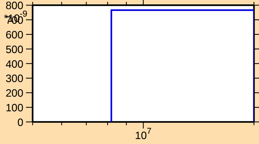
\sigma vs. E for ^{135}\text{Gd}(n,2np)
