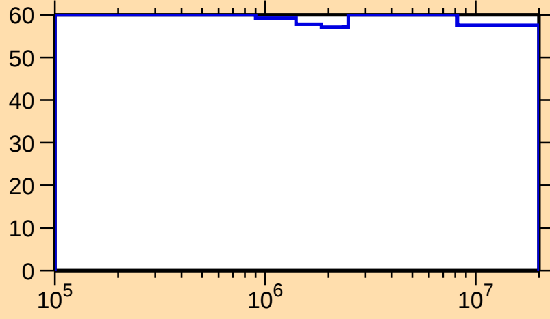
\Delta\sigma/\sigma vs. E for ^{135}\text{Gd}(n,n_1)
