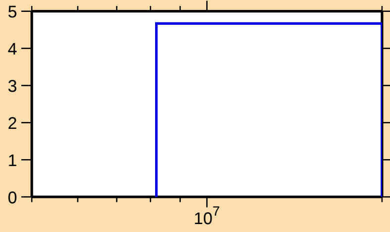
\Delta\sigma/\sigma vs. E for ^{135}\text{Gd}(n,\text{nonel.})
