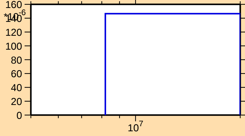
\sigma vs. E for ^{135}\text{Gd}(n,\text{pt})
