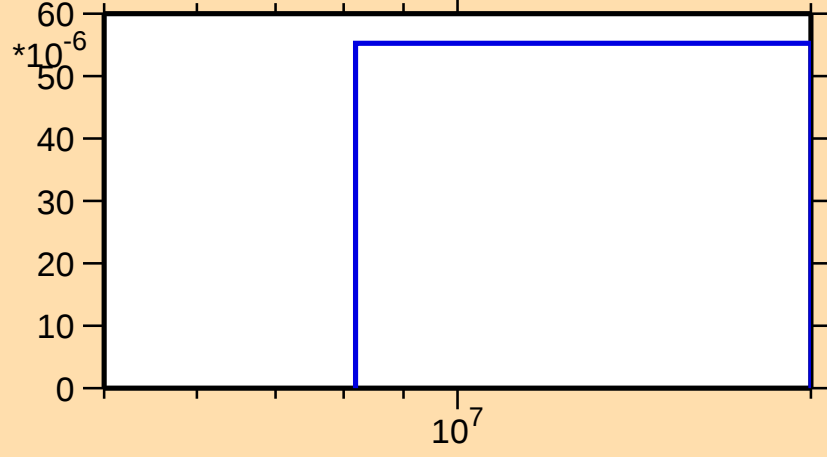
\sigma vs. E for ^{135}\text{Gd}(n,2n)
