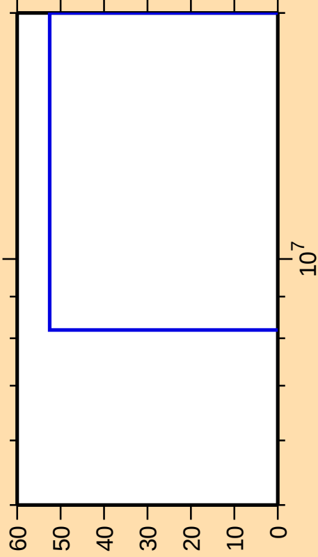
\Delta\sigma/\sigma vs. E for ^{135}\text{Gd}(n,2np)
