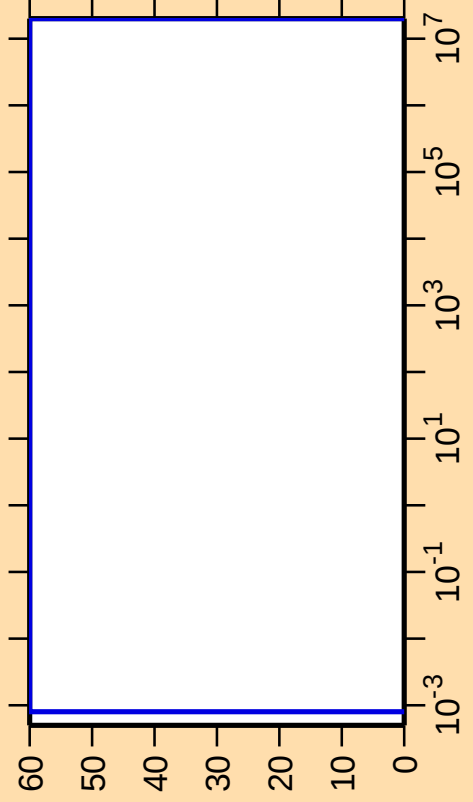
\Delta\sigma/\sigma vs. E for ^{135}\text{Gd}(n,\alpha)
