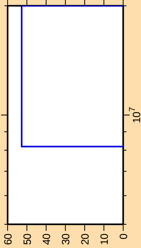
\Delta\sigma/\sigma vs. E for ^{135}\text{Gd}(n,n_{\text{cont}})
