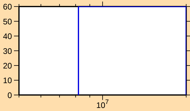
\Delta\sigma/\sigma vs. E for ^{135}\text{Gd}(n,2n)
