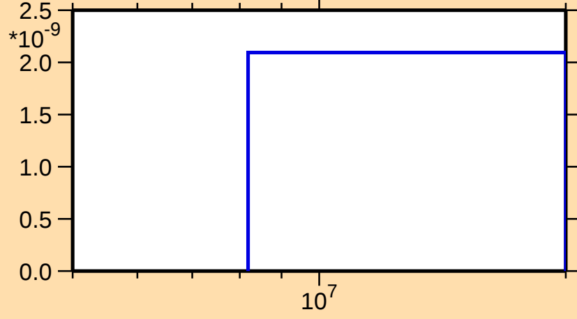
\sigma vs. E for ^{135}\text{Gd}(n,\text{nd})
