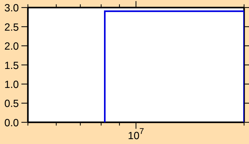
\Delta\sigma/\sigma vs. E for ^{135}\text{Gd}(n,\text{tot.})
