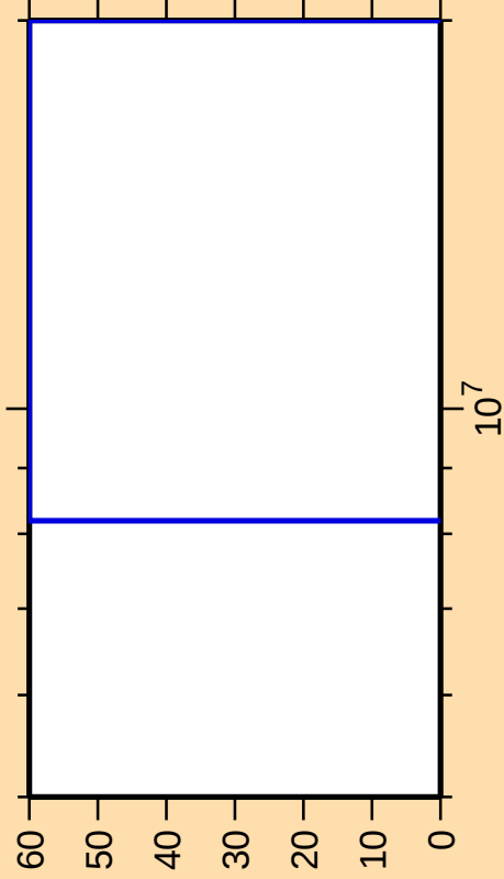
\Delta\sigma/\sigma vs. E for ^{135}\text{Gd}(\text{mt117})
