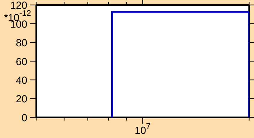
\sigma vs. E for ^{135}\text{Gd}(n,2n\alpha)
