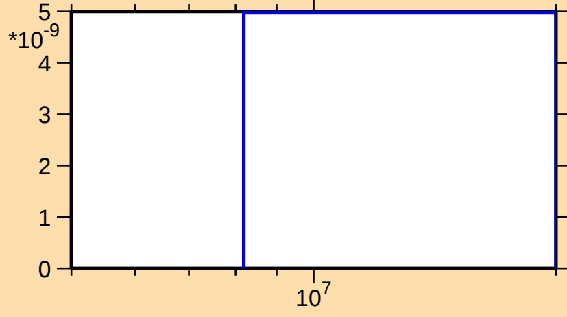
\sigma vs. E for ^{135}\text{Gd}(\text{mt } 34)
