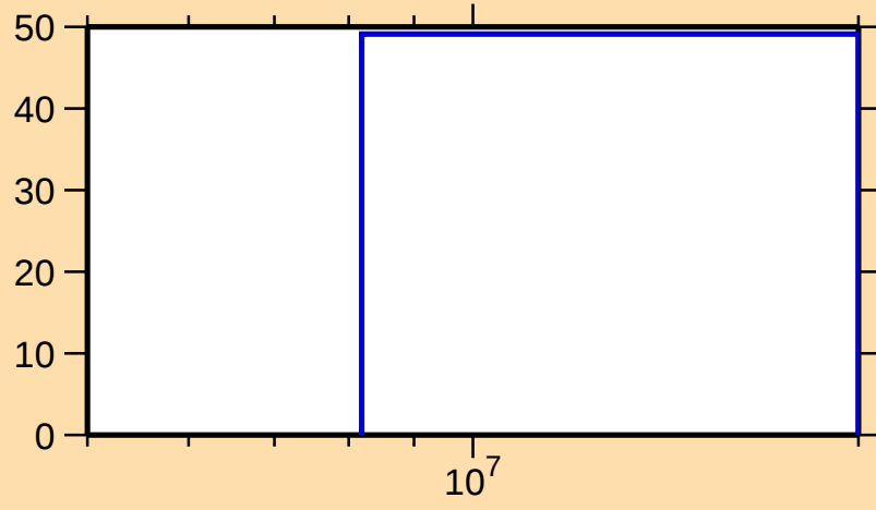
\Delta\sigma/\sigma vs. E for ^{135}\text{Gd}(n,\text{inel.})
