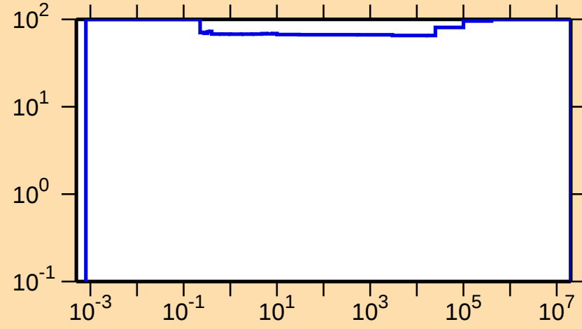
\Delta\sigma/\sigma vs. E for ^{135}\text{Gd}(n,p)
