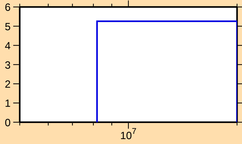
\Delta\sigma/\sigma vs. E for ^{135}\text{Gd}(n,\text{el.})
