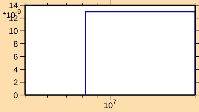
\sigma vs. E for ^{135}\text{Gd}(\text{mt117})
