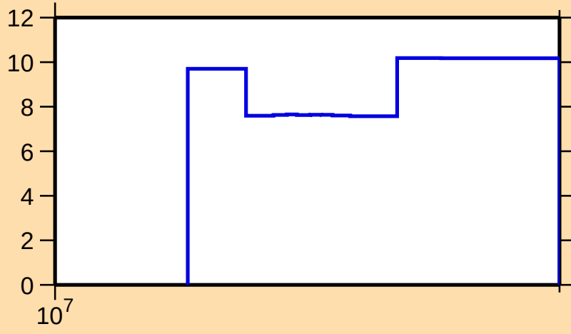
\Delta\sigma/\sigma vs. E for ^{136}\text{Gd}(n,\text{el.})
