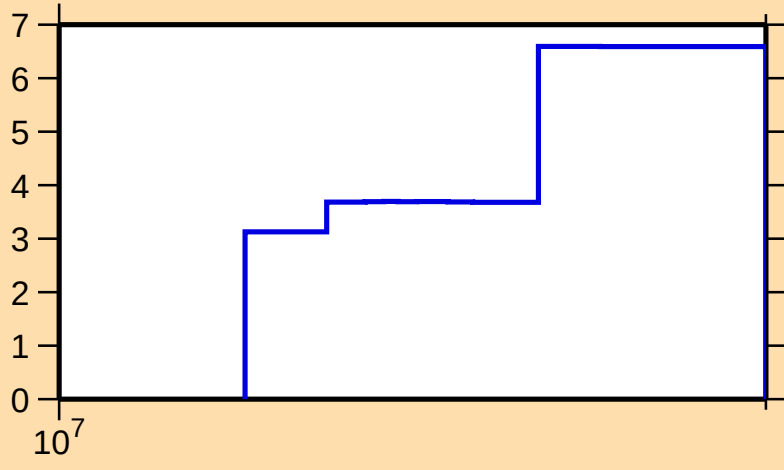
\Delta\sigma/\sigma vs. E for ^{136}\text{Gd}(n,\text{tot.})
