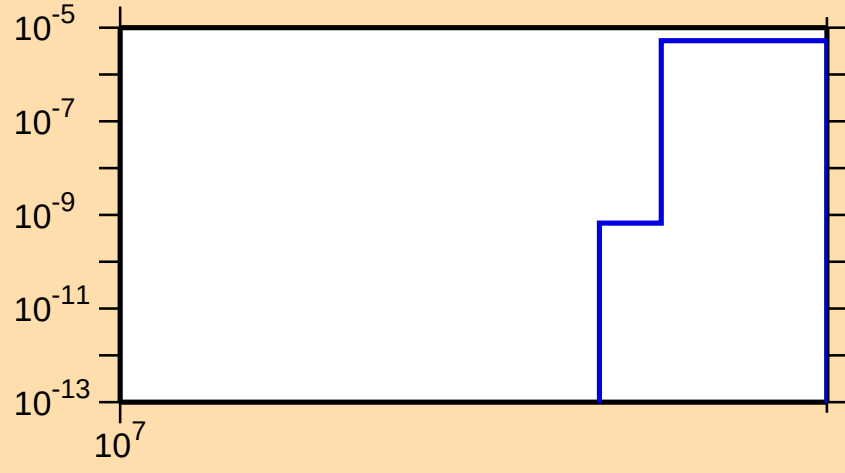
\sigma vs. E for ^{136}\text{Gd}(n,2np)
