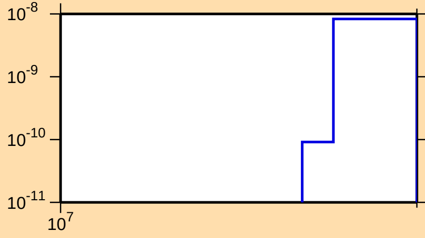
\sigma vs. E for ^{136}\text{Gd}(n,\text{nd})
