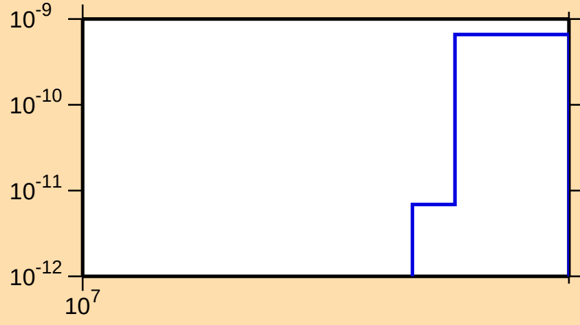
\sigma vs. E for ^{136}\text{Gd}(n,2n\alpha)
