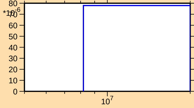
\sigma vs. E for ^{136}\text{Gd}(n,t)
