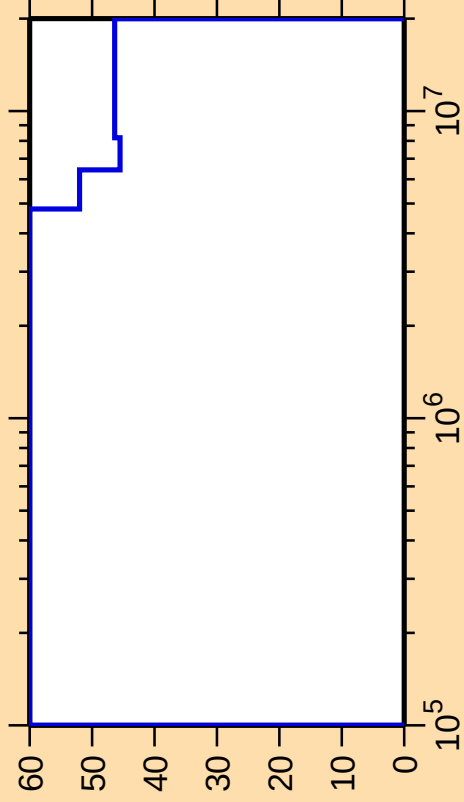
\Delta\sigma/\sigma vs. E for ^{136}\text{Gd}(n,\text{inel.})
