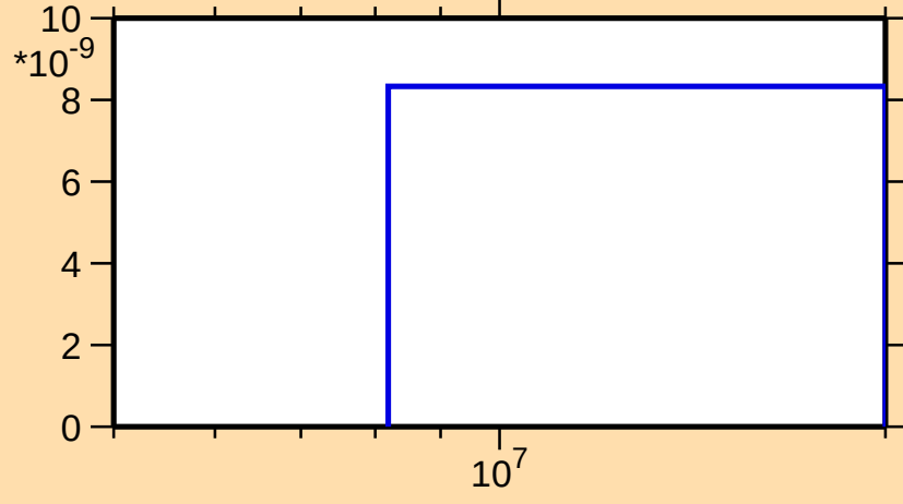
\sigma vs. E for ^{136}\text{Gd}(\text{mt117})
