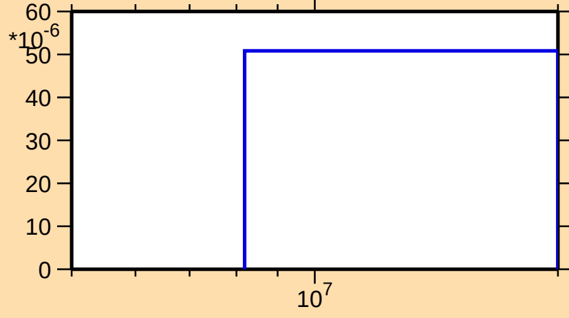
\sigma vs. E for ^{136}\text{Gd}(n,2n)
