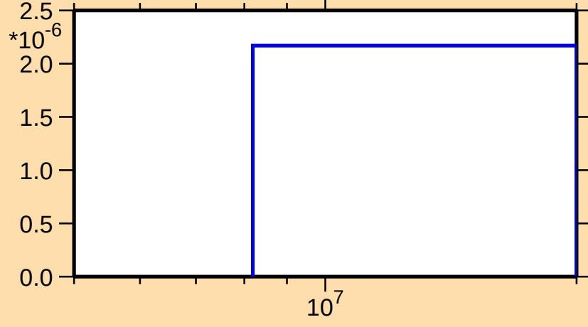
\sigma vs. E for ^{136}\text{Gd}(n,\text{pt})
