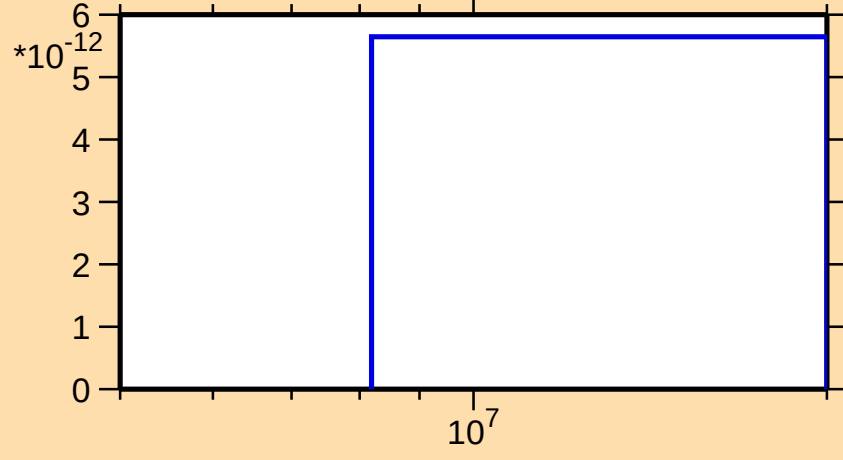
\sigma vs. E for ^{136}\text{Gd}(n,2n\alpha)
