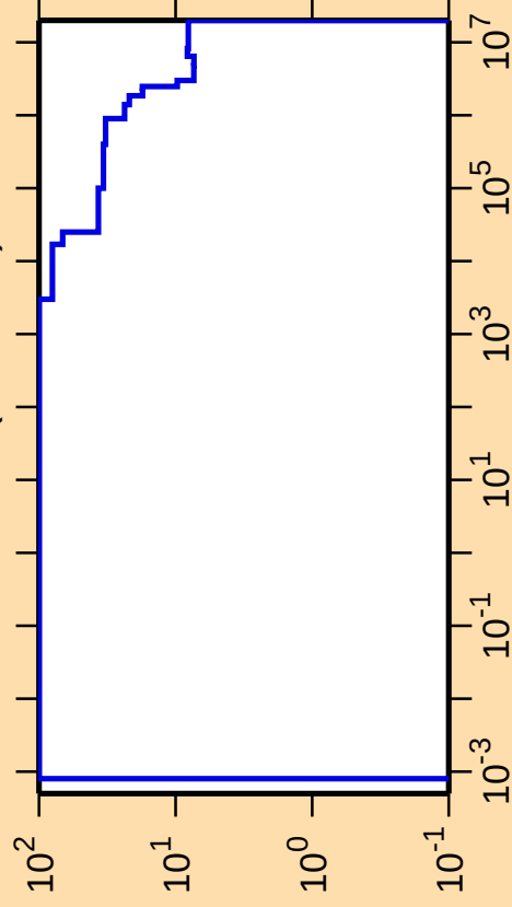
\Delta\sigma/\sigma vs. E for ^{136}\text{Gd}(n,\text{nonel.})
