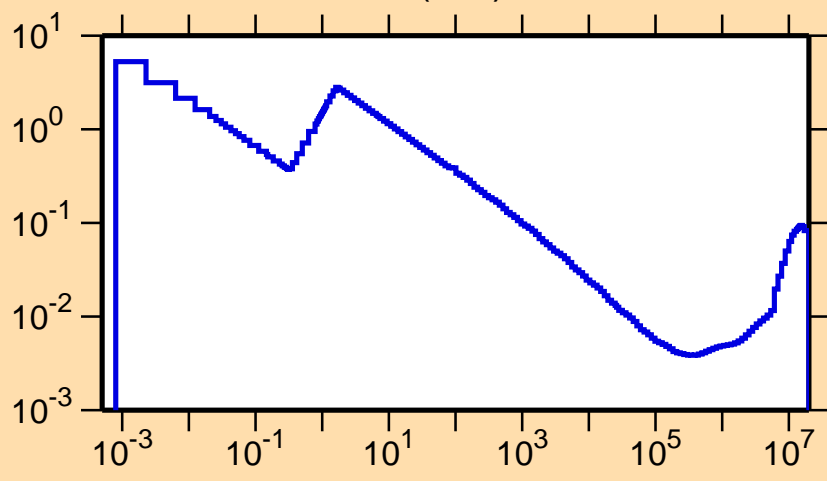
\sigma vs. E for ^{138}\text{Gd}(n,\alpha)
