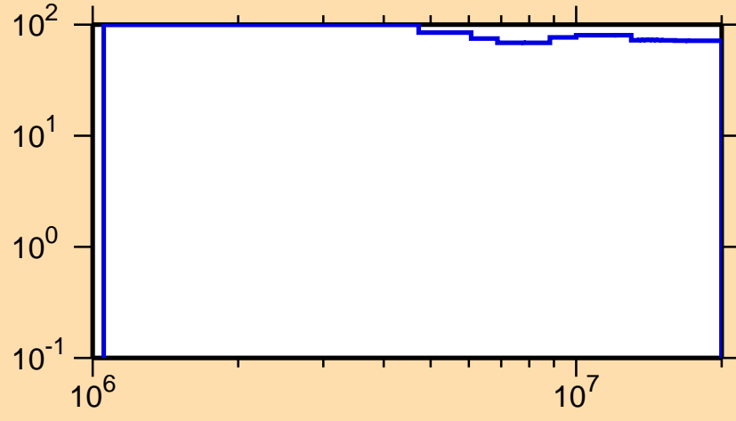
\Delta\sigma/\sigma vs. E for ^{138}\text{Gd}(n,n\text{cont.})
