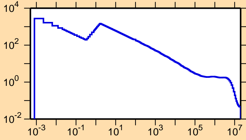
\sigma vs. E for ^{138}\text{Gd}(n,p)
