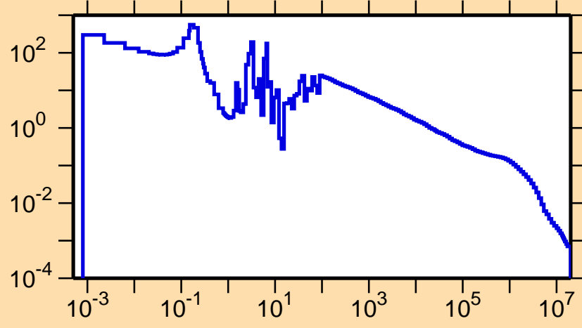
\sigma vs. E for ^{138}\text{Gd}(n,\gamma)
