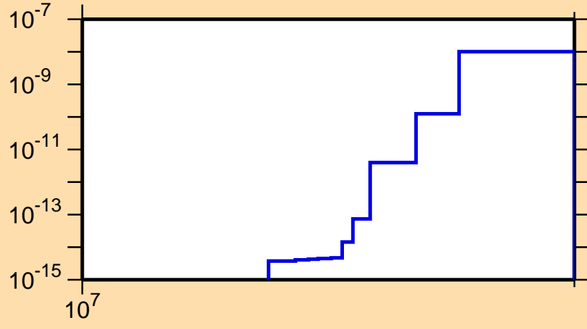
\sigma vs. E for ^{138}\text{Gd}(n,2n\alpha)
