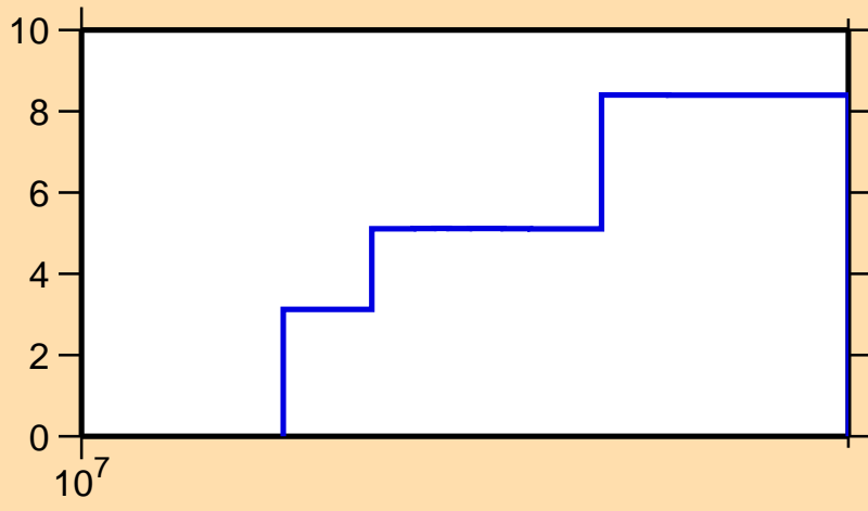
\Delta\sigma/\sigma vs. E for ^{138}\text{Gd}(n,\text{tot.})
