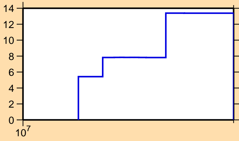
\Delta\sigma/\sigma vs. E for ^{138}\text{Gd}(n,\text{el.})
