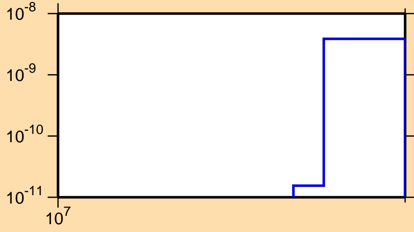
\sigma vs. E for ^{138}\text{Gd}(n,\text{nd})
