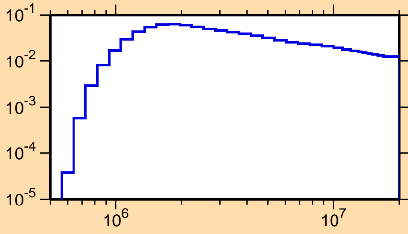
\sigma vs. E for ^{138}\text{Gd}(n,n_2)
