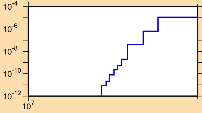
\sigma vs. E for ^{138}\text{Gd}(n,\text{pt})
