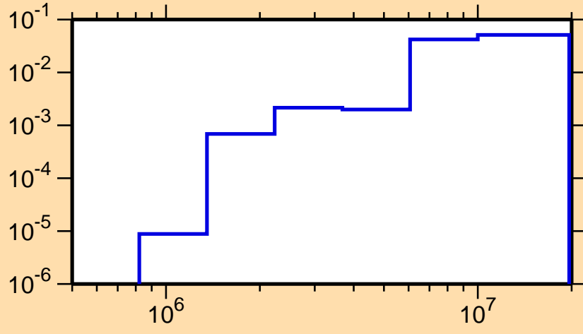
\sigma vs. E for ^{138}\text{Gd}(n,n\text{cont.})
