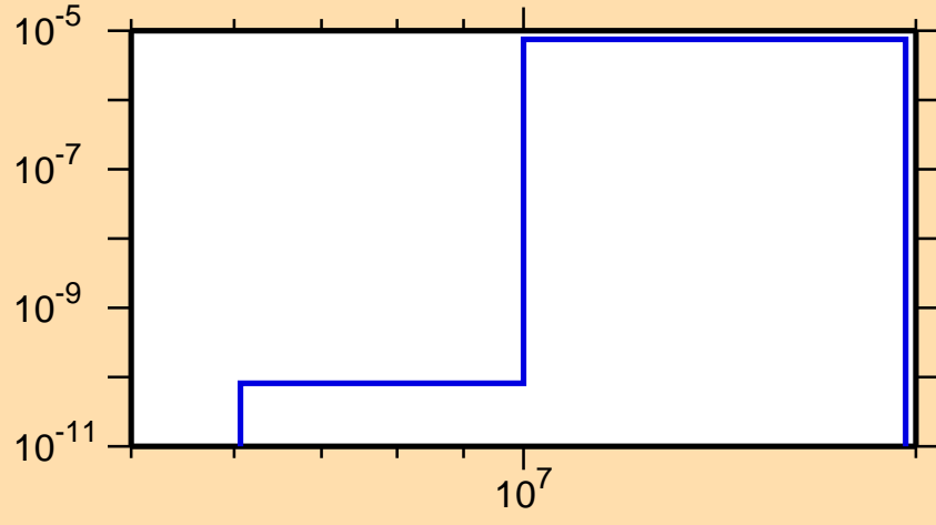
\sigma vs. E for ^{138}\text{Gd} (mt 45)
