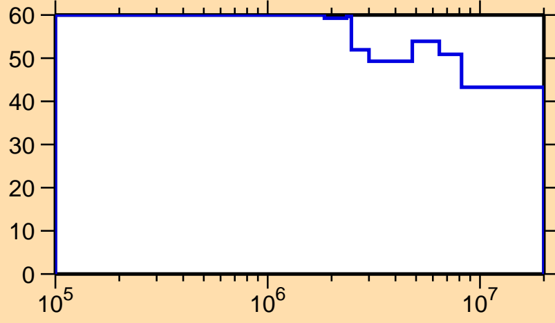
\Delta\sigma/\sigma vs. E for ^{138}\text{Gd}(n,n_1)
