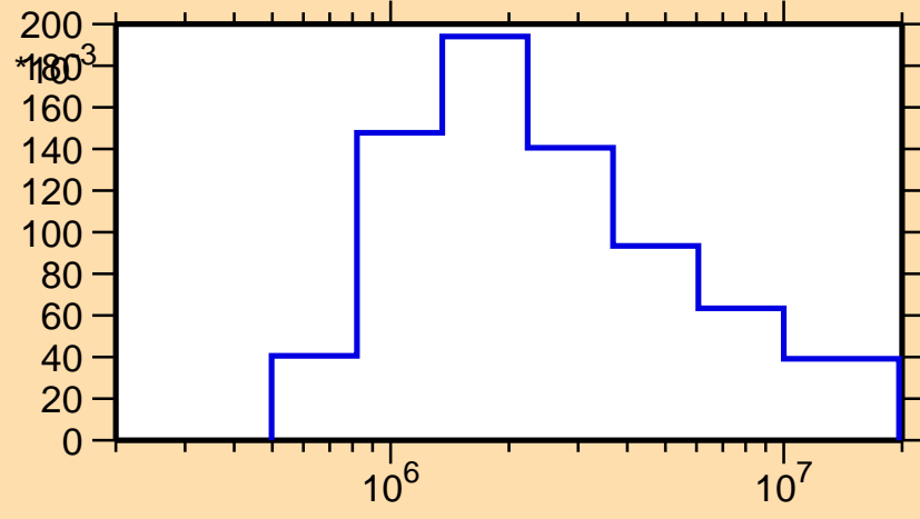
\sigma vs. E for ^{139}\text{Gd}(n,n_4)
