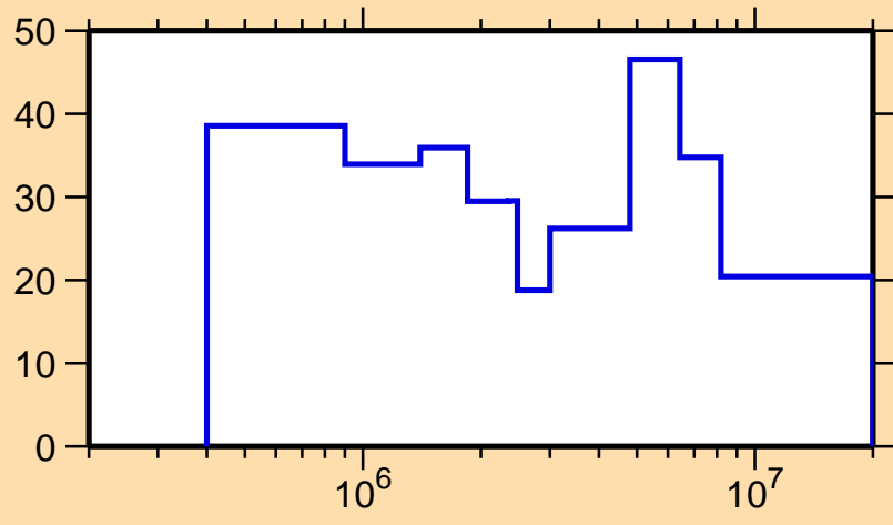
\Delta\sigma/\sigma vs. E for ^{139}\text{Gd}(n,\text{el.})
