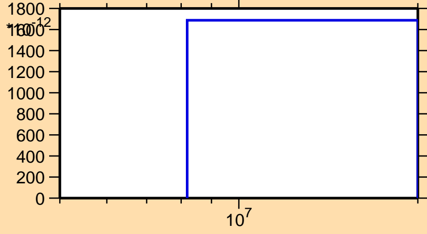
\sigma vs. E for ^{139}\text{Gd} (mt 34)
