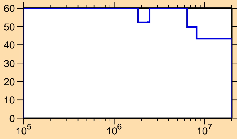
\Delta\sigma/\sigma vs. E for ^{139}\text{Gd}(n,n_1)
