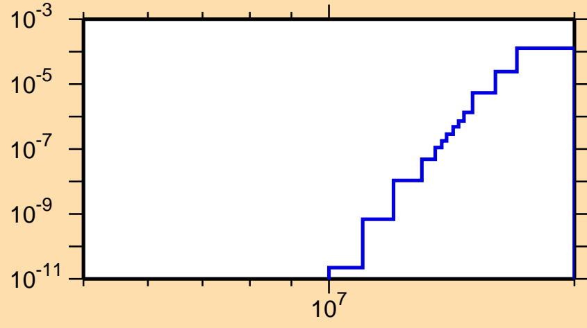
\sigma vs. E for ^{139}\text{Gd} (mt 45)
