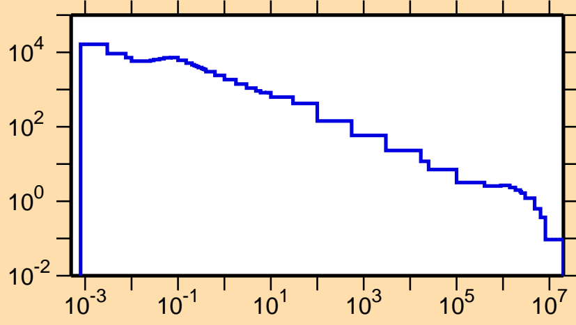
\sigma vs. E for ^{139}\text{Gd}(n,p)
