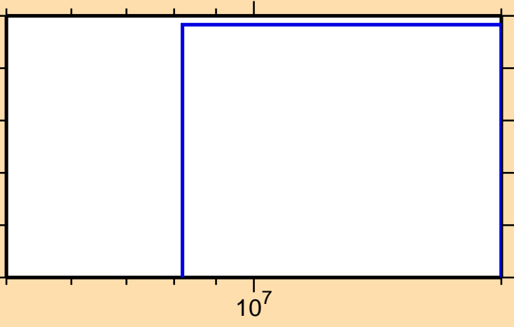
\sigma vs. E for ^{139}\text{Gd}(\text{mt117})
