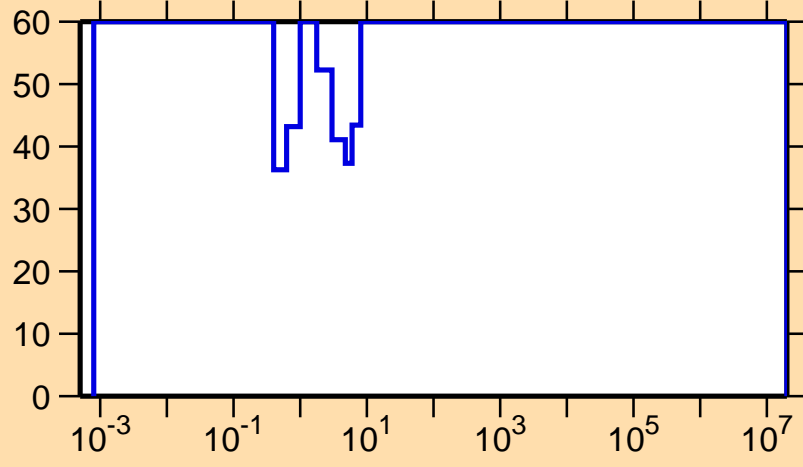
\Delta\sigma/\sigma vs. E for ^{139}\text{Gd}(n,\gamma)
