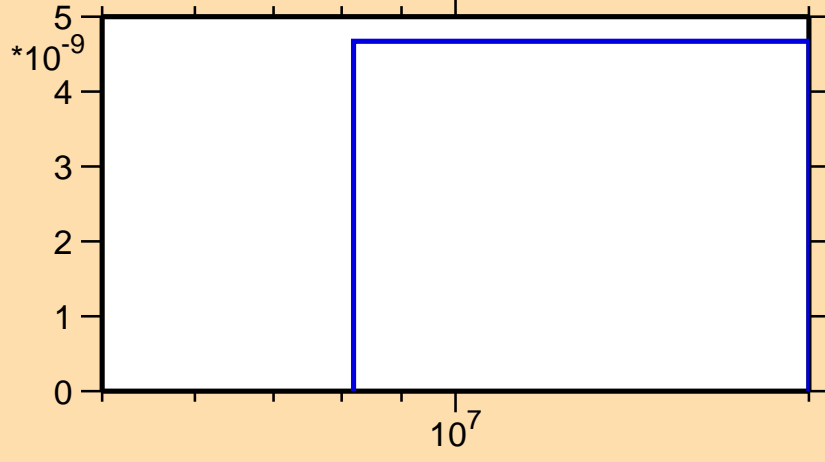
\sigma vs. E for ^{139}\text{Gd} (mt 34)
