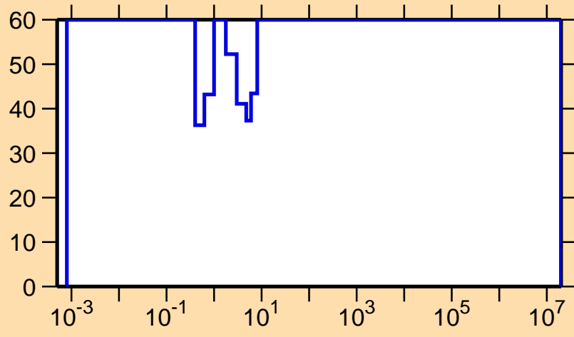
\Delta\sigma/\sigma vs. E for ^{139}\text{Gd}(n,\gamma)
