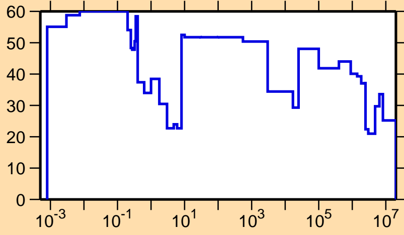
\Delta\sigma/\sigma vs. E for ^{139}\text{Gd}(n,\text{tot.})
