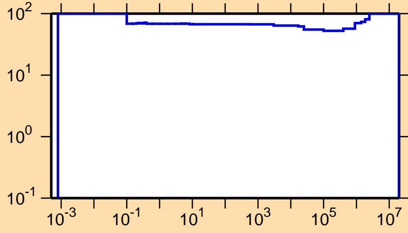
\Delta\sigma/\sigma vs. E for ^{139}\text{Gd}(n,p)
