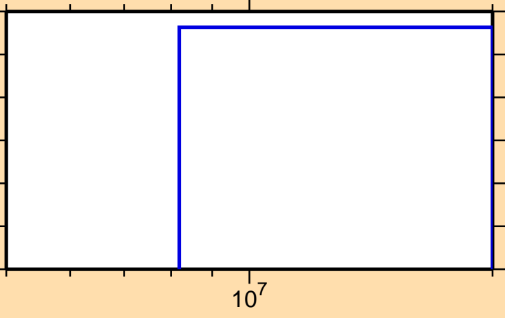
\sigma vs. E for ^{139}\text{Gd}(n,\text{nd})
