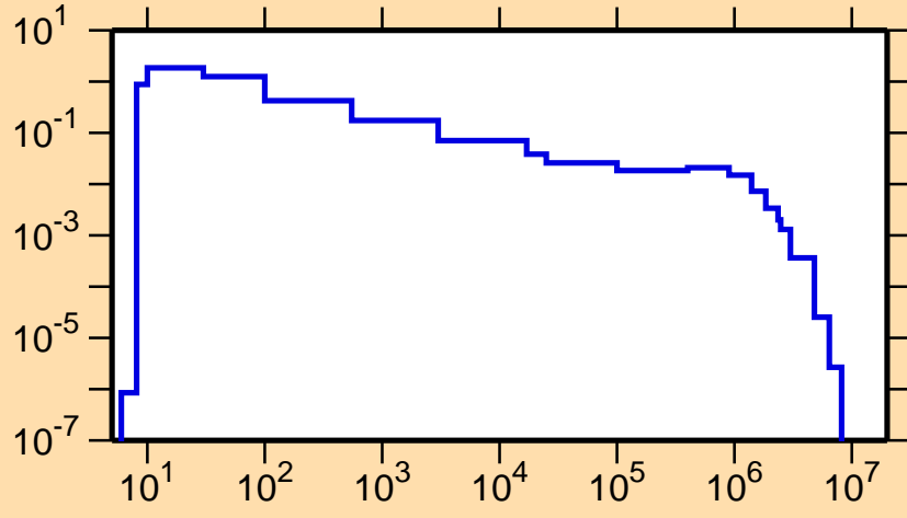
\sigma vs. E for ^{139}\text{Gd}(n,n_1)
