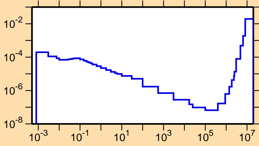
\sigma vs. E for ^{139}\text{Gd}(n,p\alpha)
