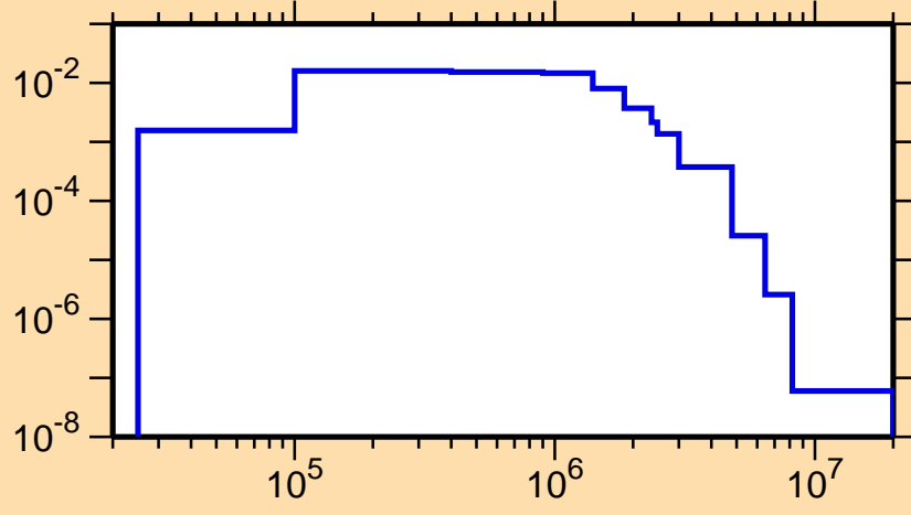
\sigma vs. E for ^{139}\text{Gd}(n,n_3)
