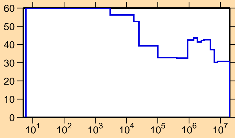
\Delta\sigma/\sigma vs. E for ^{139}\text{Gd}(n,\text{nonel.})
