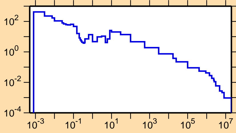
\sigma vs. E for ^{139}\text{Gd}(n,\gamma)
