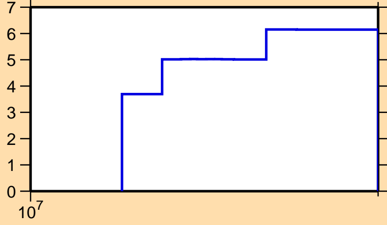
\Delta\sigma/\sigma vs. E for ^{140}\text{Gd}(n,\text{el.})
