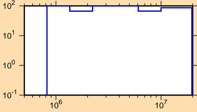
\Delta\sigma/\sigma vs. E for ^{140}\text{Gd}(n,n\text{cont.})
