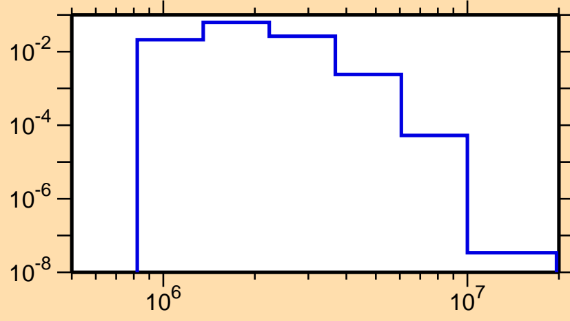
\sigma vs. E for ^{140}\text{Gd}(n,n_4)
