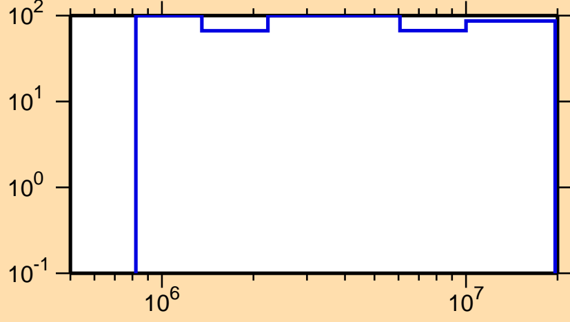
\Delta\sigma/\sigma vs. E for ^{140}\text{Gd}(n,ncont.)
