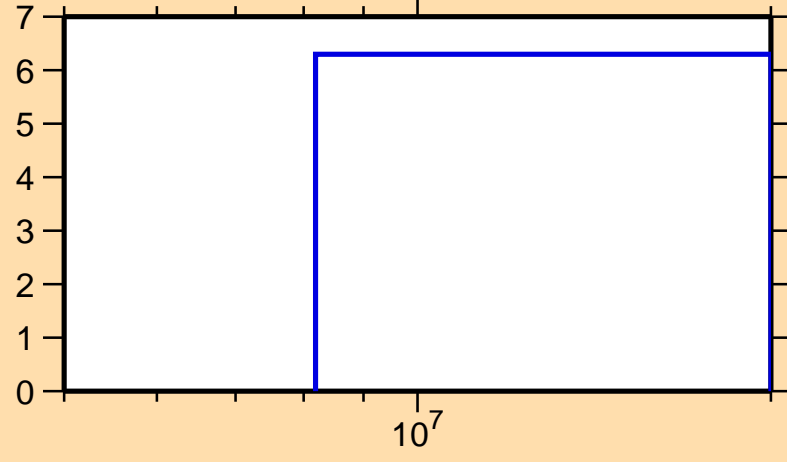
\Delta\sigma/\sigma vs. E for ^{140}\text{Gd}(n,\text{nonel.})
