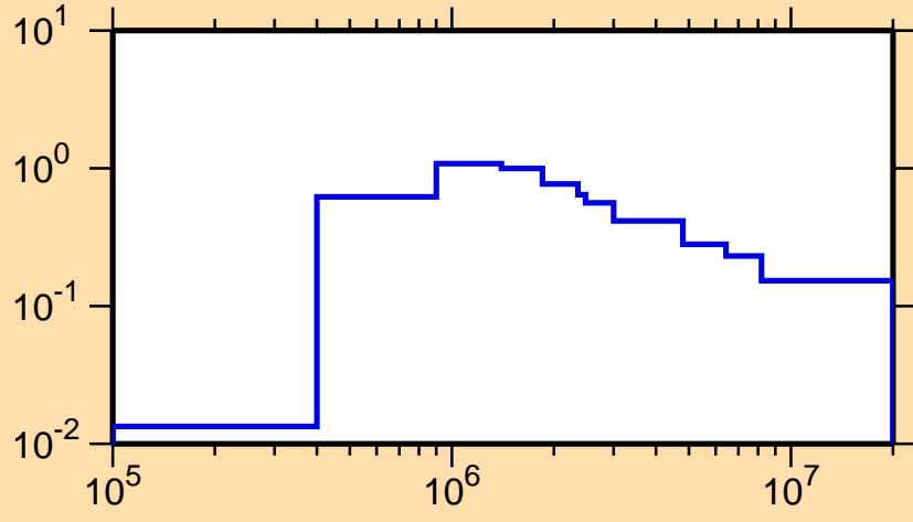
\sigma vs. E for ^{140}\text{Gd}(n,n_1)
