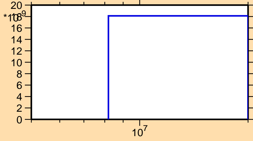
\sigma vs. E for ^{140}\text{Gd}(n,2np)
