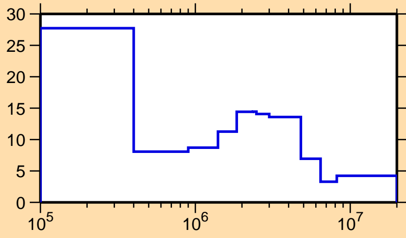
\Delta\sigma/\sigma vs. E for ^{140}\text{Gd}(n,\text{el.})
