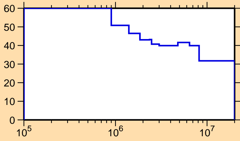
\Delta\sigma/\sigma vs. E for ^{140}\text{Gd}(n,n_1)
