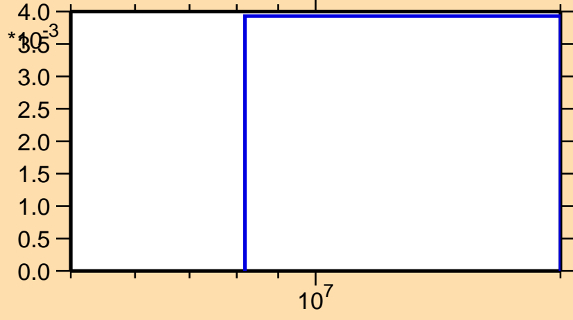
\sigma vs. E for ^{140}\text{Gd}(n,2n)
