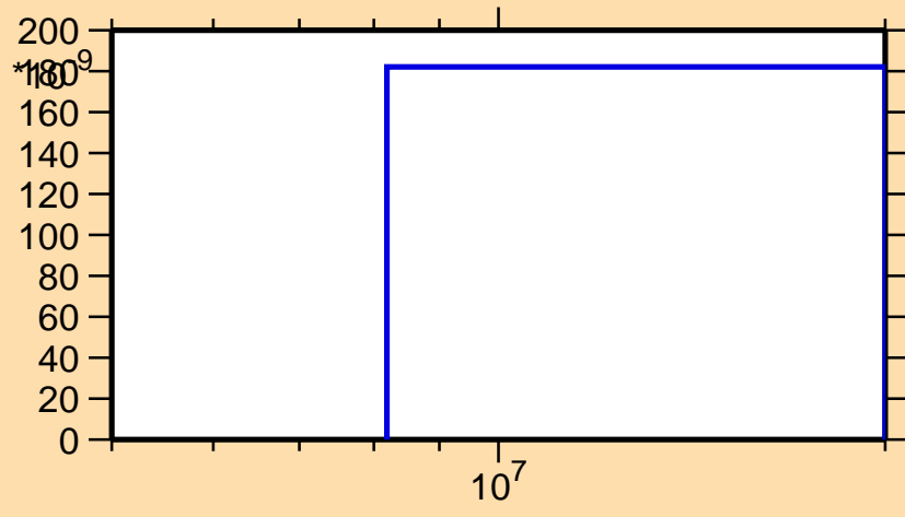
\sigma vs. E for ^{140}\text{Gd}(\text{mt } 45)
