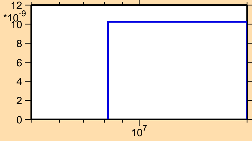
\sigma vs. E for ^{140}\text{Gd}(n,\text{pt})
