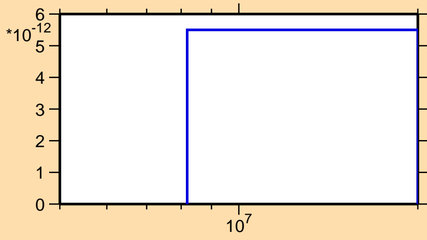
\sigma vs. E for ^{140}\text{Gd} (mt 34)
