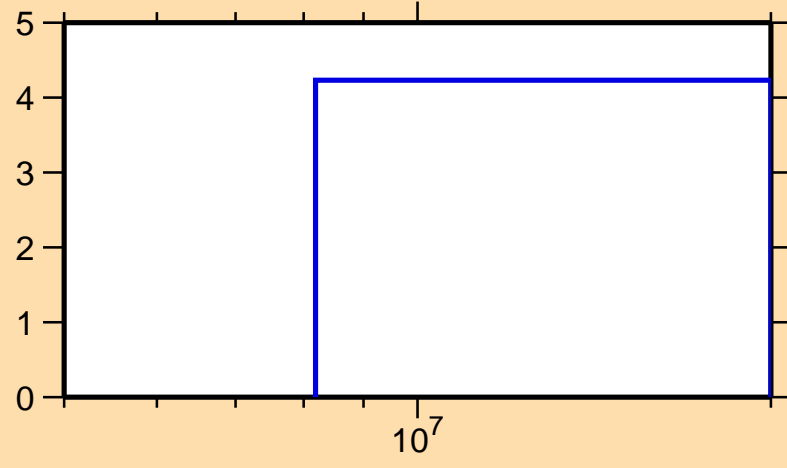
\Delta\sigma/\sigma vs. E for ^{140}\text{Gd}(n,\text{el.})
