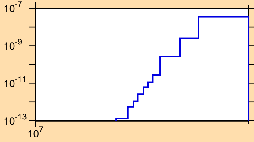
\sigma vs. E for ^{141}\text{Gd} (mt 34)
