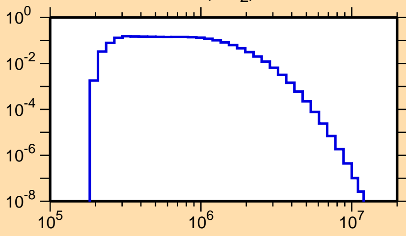
\sigma vs. E for ^{141}\text{Gd}(n,n_2)
