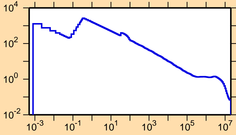
\sigma vs. E for ^{141}\text{Gd}(n,p)
