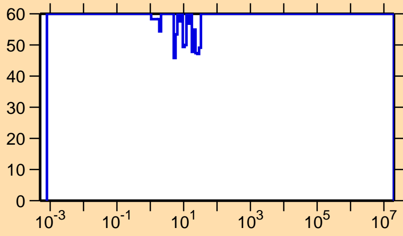
\Delta\sigma/\sigma vs. E for ^{141}\text{Gd}(n,\gamma)
