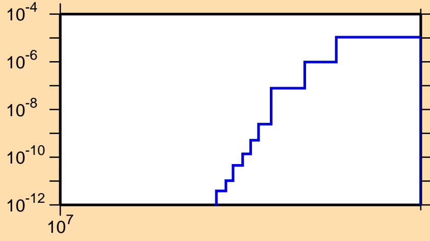
\sigma vs. E for ^{141}\text{Gd}(n,\text{nd})
