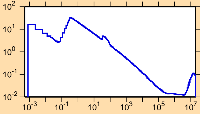
\sigma vs. E for ^{141}\text{Gd}(n,\alpha)
