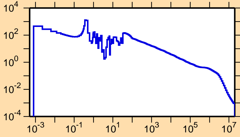
\sigma vs. E for ^{141}\text{Gd}(n,\gamma)
