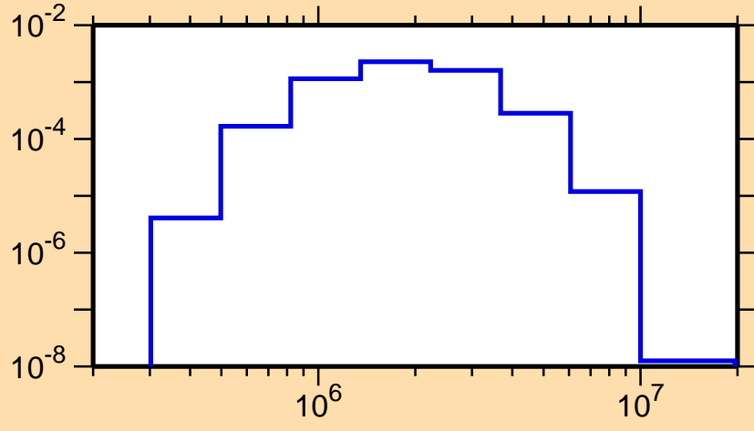
\sigma vs. E for ^{141}\text{Gd}(n,n_4)
