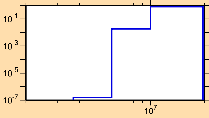
\sigma vs. E for ^{141}\text{Gd}(n,np)
